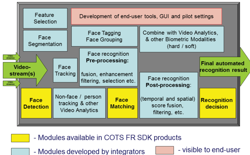
Figure 1: Face processing tasks required for integration of FR solutions into a video surveillance application.
