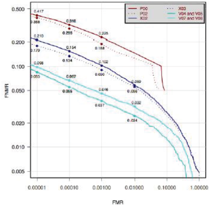
Figure 2: The Detection Error Tradeoff (DET) curves for NEC, Cognitec and PittPat products (from NIST Multiple-Biometric Evaluation ).
