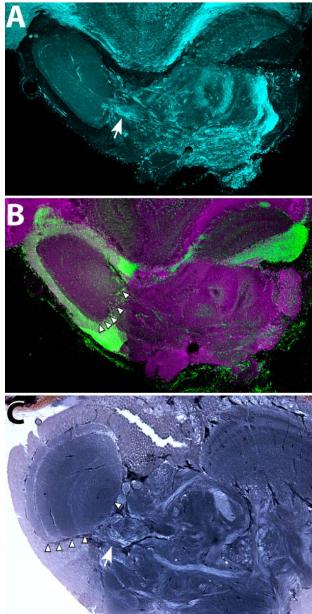
Figure 3. The elaborate S. empusa hemiellipsoid body. The crustacean hemiellipsoid body is evolutionarily homologous with the mushroom body of insects, which has been shown to be essential for olfactory learning and memory and spatial navigation. Unlike other crustaceans that have a hemiellipsoid body consisting of merely 2 subunits, the stomatopod hemiellipsoid body is greatly enlarged in size and further divided into at least 5 distinct layers (arrowheads in B , C ). This organization is much similar to the mushroom body of honey bees, of which is also enlarged and divided into distinct regions that receive segregated neural inputs from visual, olfactory, and mechanosensory centers. Distinct output fibers originating from the stomatopod hemiellipsoid body can be seen (arrows in A , C ). This is unique among all crustacean hemiellipsoid bodies. A and B , immunoreactivity against \alpha -tubulin (cyan) and synapsin (pink), and nuclear stain showing the cell bodies (green). C , nuclear stain showing the cell bodies (green).
