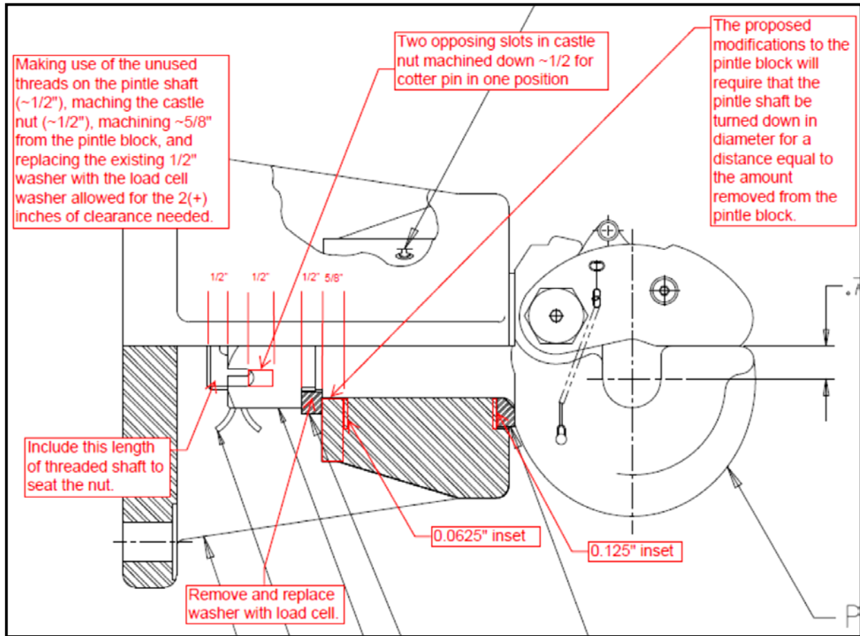
Figure 1. Pintle assembly modifications diagram - M88A2.
