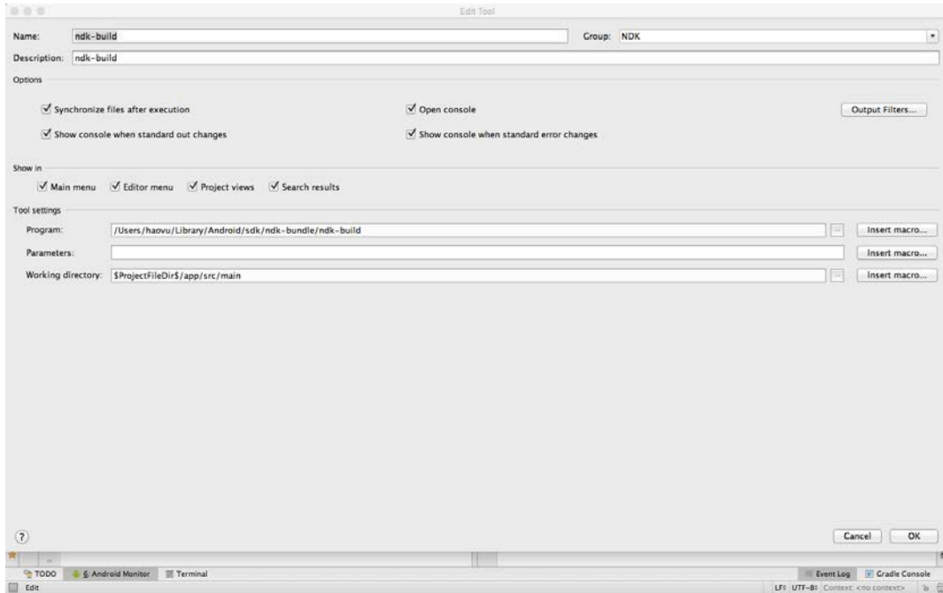
Fig. 3 Environment path
