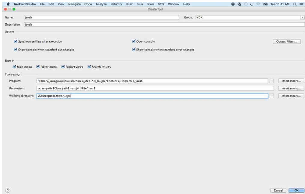
Fig. 2 “Javah” path
