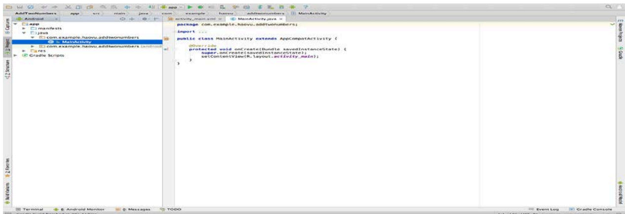
Fig. 5 Android application
