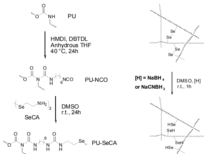
Figure 1. The synthesis scheme used to prepare polyurethanes possessing covalently appended RSe catalytic sites.
