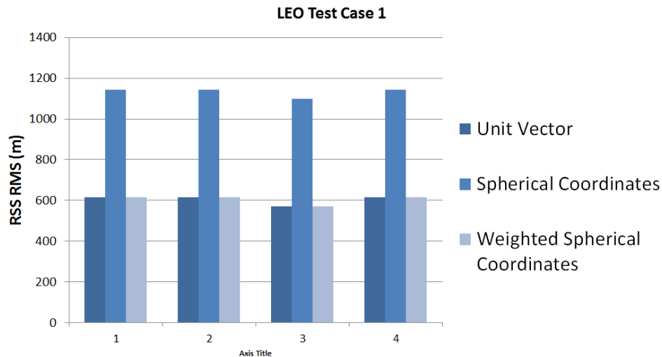
Figure 4: LEO test case 1 ephemeris difference.
