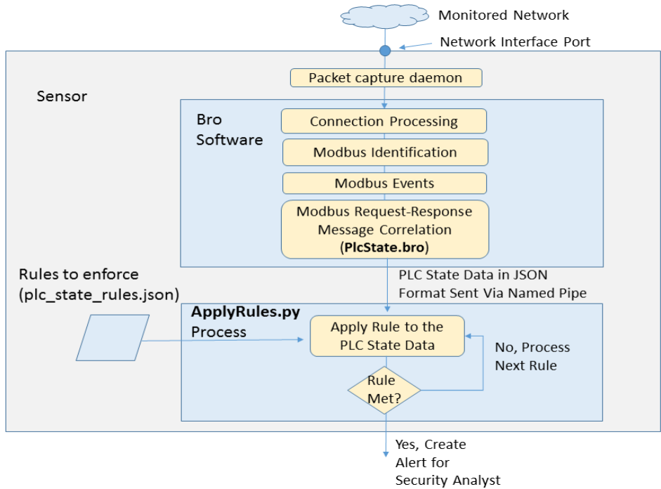
Fig. 2 iPoid components on a sensor
