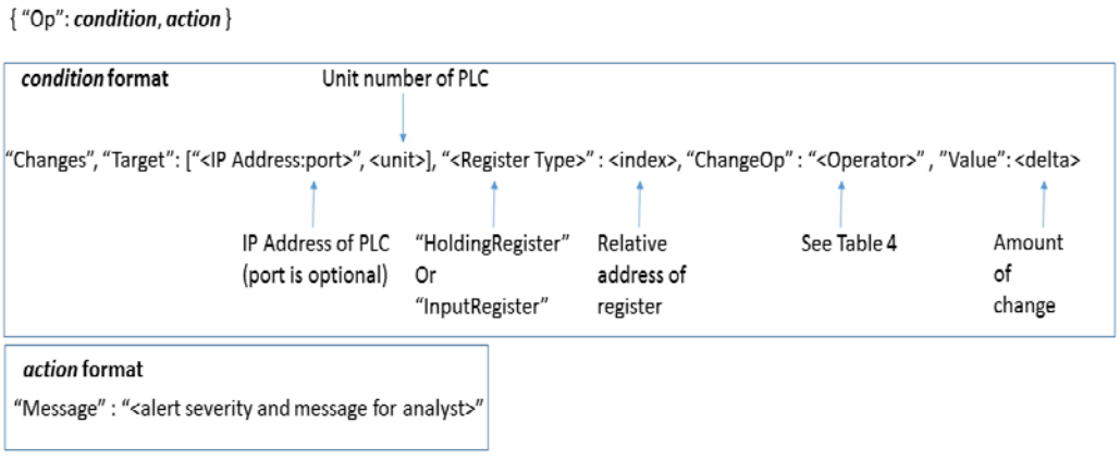
Fig. 6 Value-rule structure to detect specified differences in register state: Use “Changes” as the <Operator> and the “ChangeOp” keyword with the delta value.
