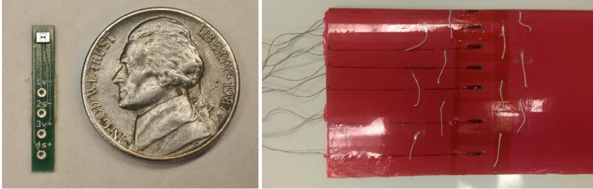
Figure 1.1 Endeveco miniature transducer (left) embedded in a test specimen (right).
