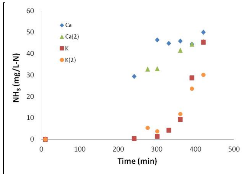
Figure 41. Effect of competing ions on ammonia sequestration (3.75 mM Ca 2+ or 1.02 mM K + ).
