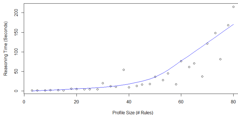
Figure 7 - Plotting the number of security requirements in the profile, versus the amount of time (in seconds) required to reason over the entire profile (and its resultant DL ontology).
