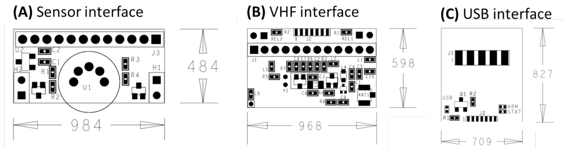
Figure 6 Three interconnect boards used to interface between the tag sub-assemblies.
