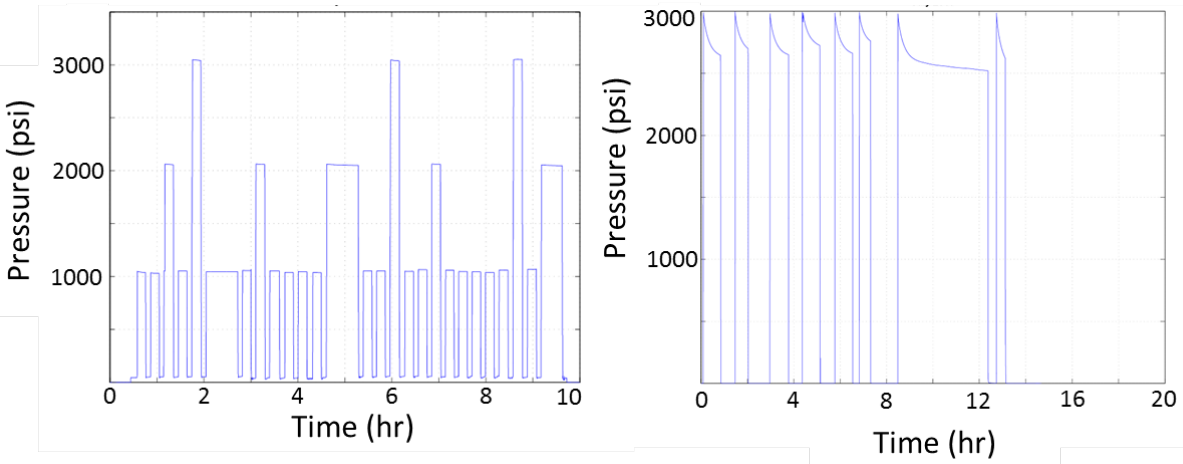
Figure 11 Representative pressure testing results from the Blake facility (left) and the Smith facility (right) that followed the Test 2 and 3 protocols respectively.
