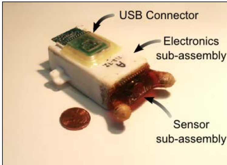
Figure 9 A picture of the combined electronics and sensor sub-assemblies used in the lab based pressure testing. Vacuum investment was used to encapsulate the electronics in epoxy.
