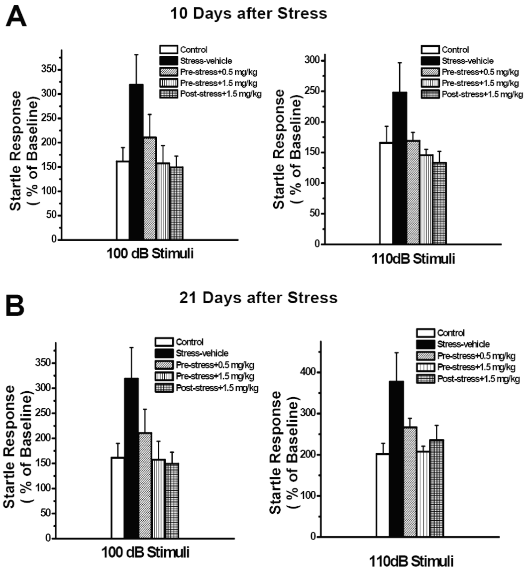
Figure 10. Mean \pm S.E.M. of peak startle amplitude (represented as % of the baseline of ASR). The groups with MDL 11,939 pretreatment and posttreatment are plotted together. The ASR to 100 dB and 110 dB was tested on both Day 10 after stress ( A ) and Day 21 after stress ( B ).
