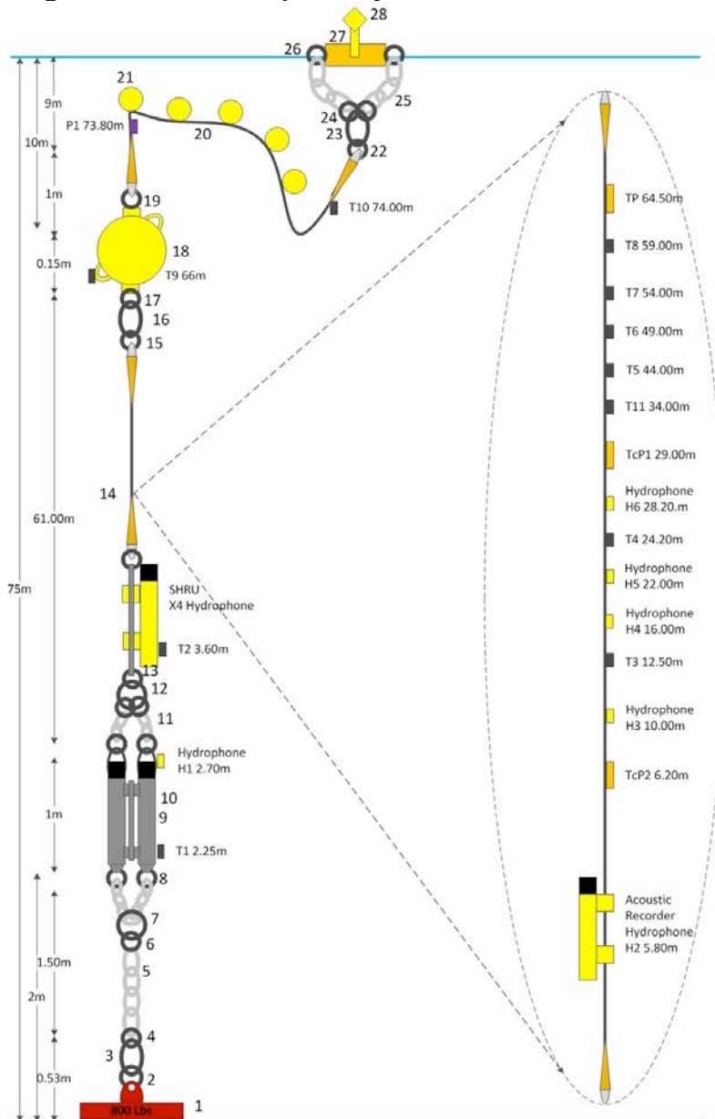
Figure 8. Mooring Configuration.
