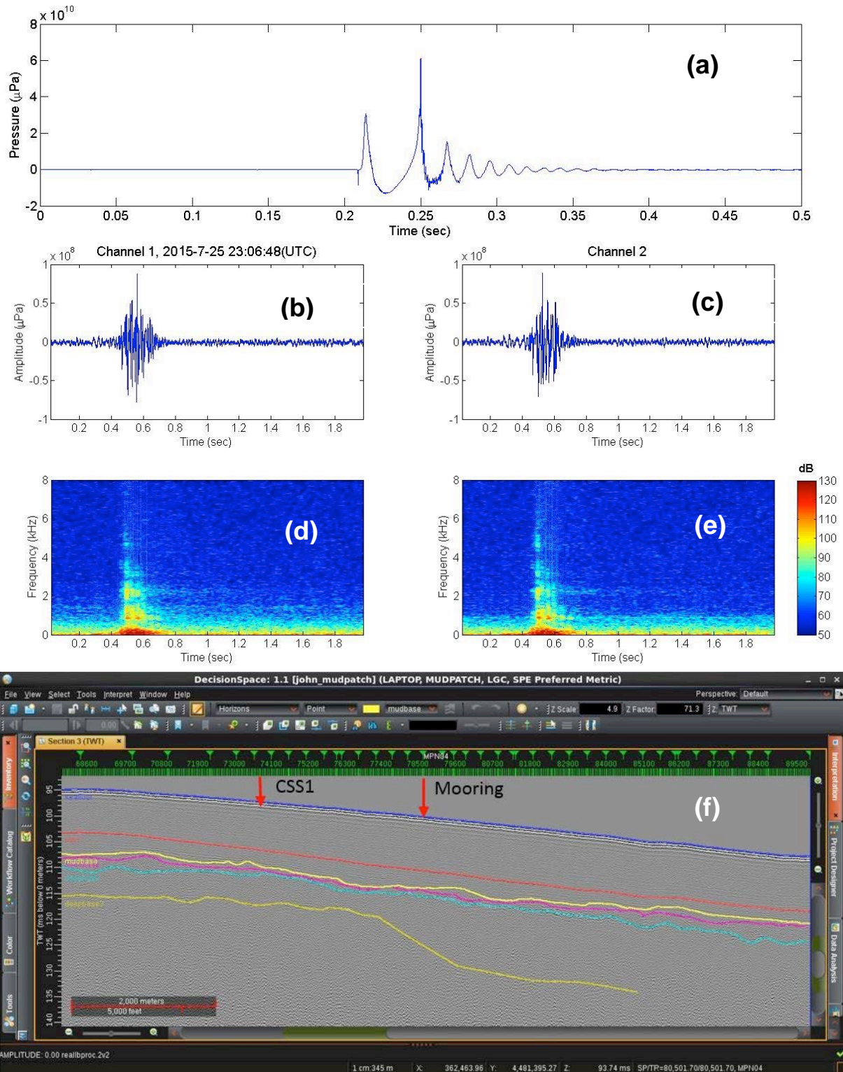
Figure 9. CSS1 ( SD=5\text{m} , \text{Range}=2.2\text{km} ) [Applied Research Lab.- UT] received by Univ. of Delaware marine recorder (2 channels). Sediment cross section plot courtesy of J. Goff [8].
