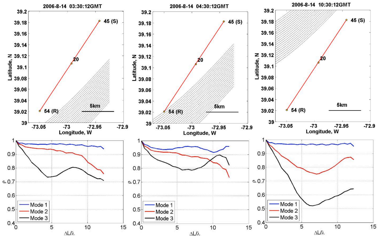
Fig. 4. The picture collage is the example showing the evolution of NLIW event 37 (first row) and the corresponding horizontal coherence of normal modes at 100Hz (second row).
