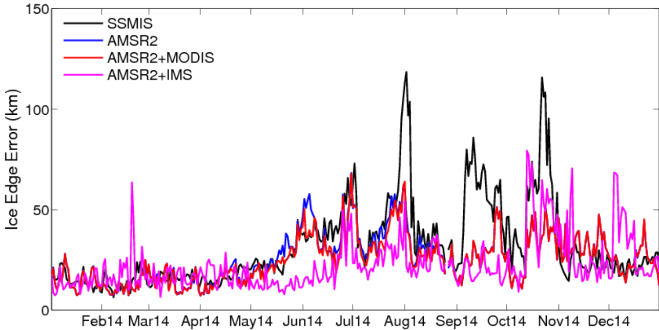
Figure 5. Daily ice edge error (km) for the Barents and Kara seas region for 2014 for SSMIS (black), AMSR2 (blue), MODIS-AMSR2 (red), and IMS-AMSR2 (magenta). Note that the y-axis range is larger than for Figure 4.
