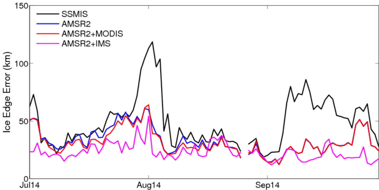
Figure 6. Daily ice edge error (km) for the Barents and Kara seas region for 14 July – 30 September 2014 for SSMIS (black), AMSR2 (blue), MODIS-AMSR2 (red), and IMS-AMSR2 (magenta).
