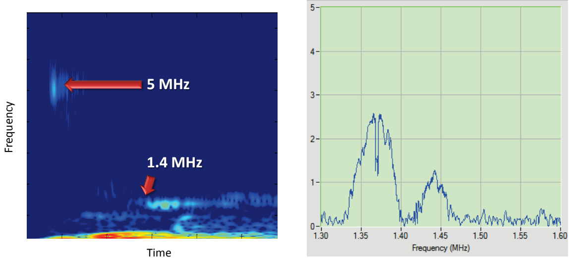
Figure 5. Two visualizations of the 1.4 Mhz mode, which is thought to be a torsional mode. The cable is tensioned to 27,000 lb and embedded in grease.
