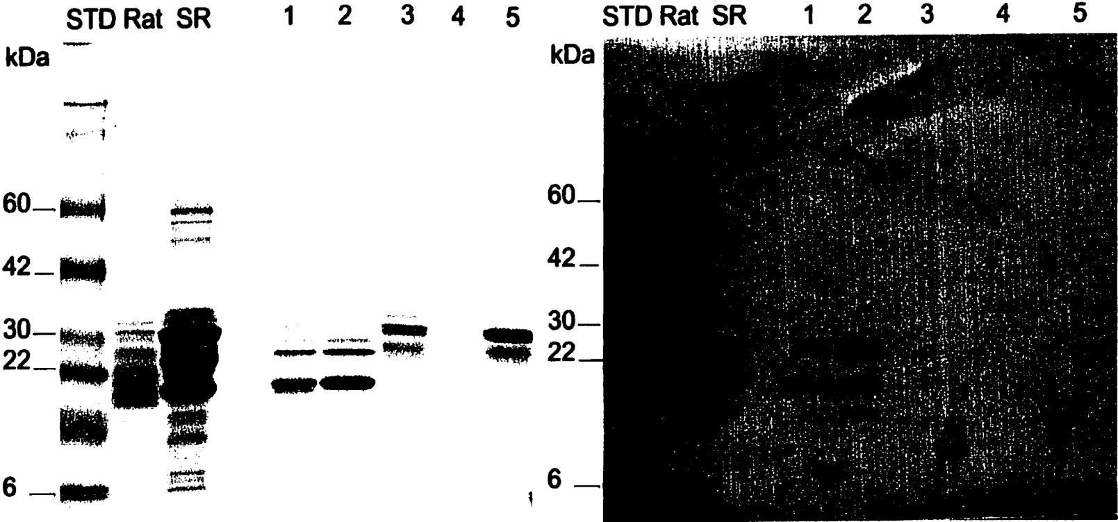
Western Blot for alpha crystallins
