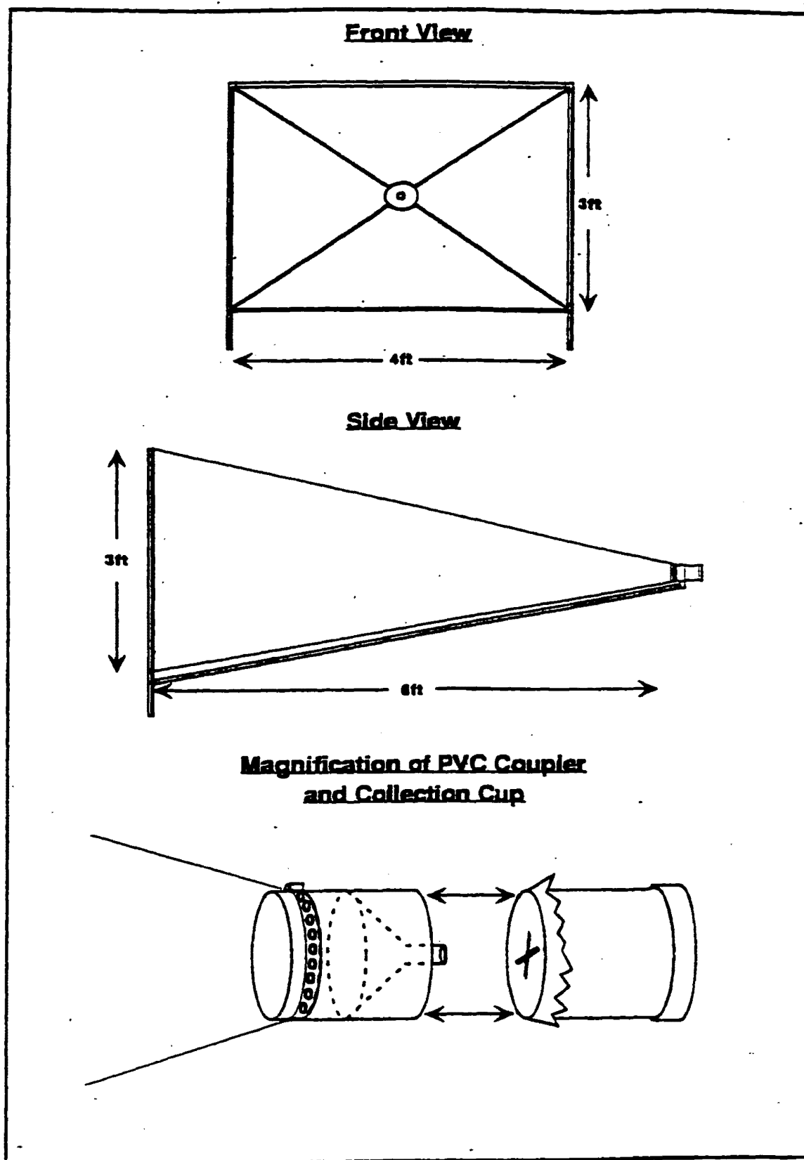
Figure 4. Illustration of the car trap and PVC coupler used for the collection of in-flight mosquito populations at the Rancho site
