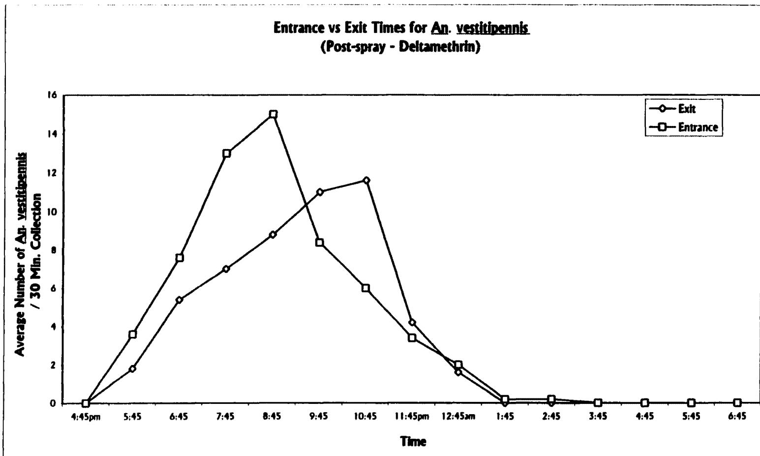
Figure 15: A comparison of entrance and exit times for Anopheles vestitipennis post-spray with deltamethrin. Entrance and exit collections were conducted on different nights. Average number of mosquitoes collected per 30-minute sample period are plotted against the midpoint of that sample period.
