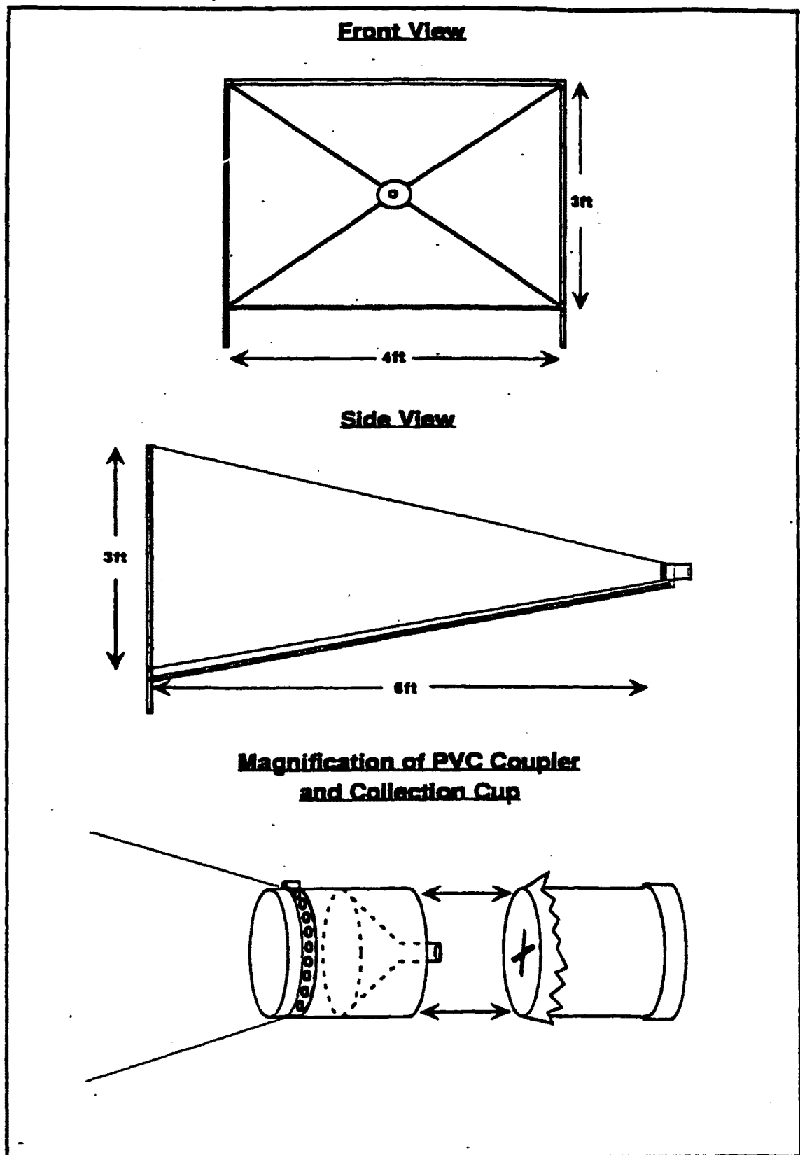
Figure 3: Illustration of the car top trap and PVC coupler used for the collection of in-flight mosquito populations at the Rancho site.
