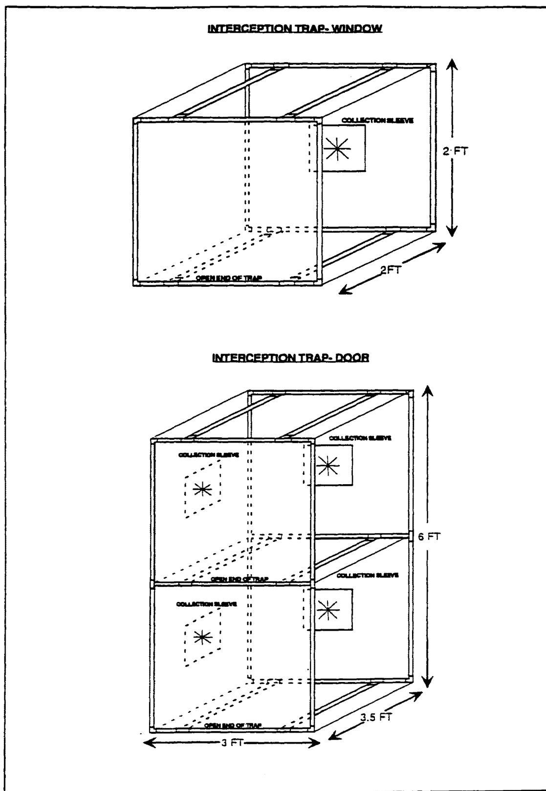
Figure 4: Illustration of the window and door intercept traps.
