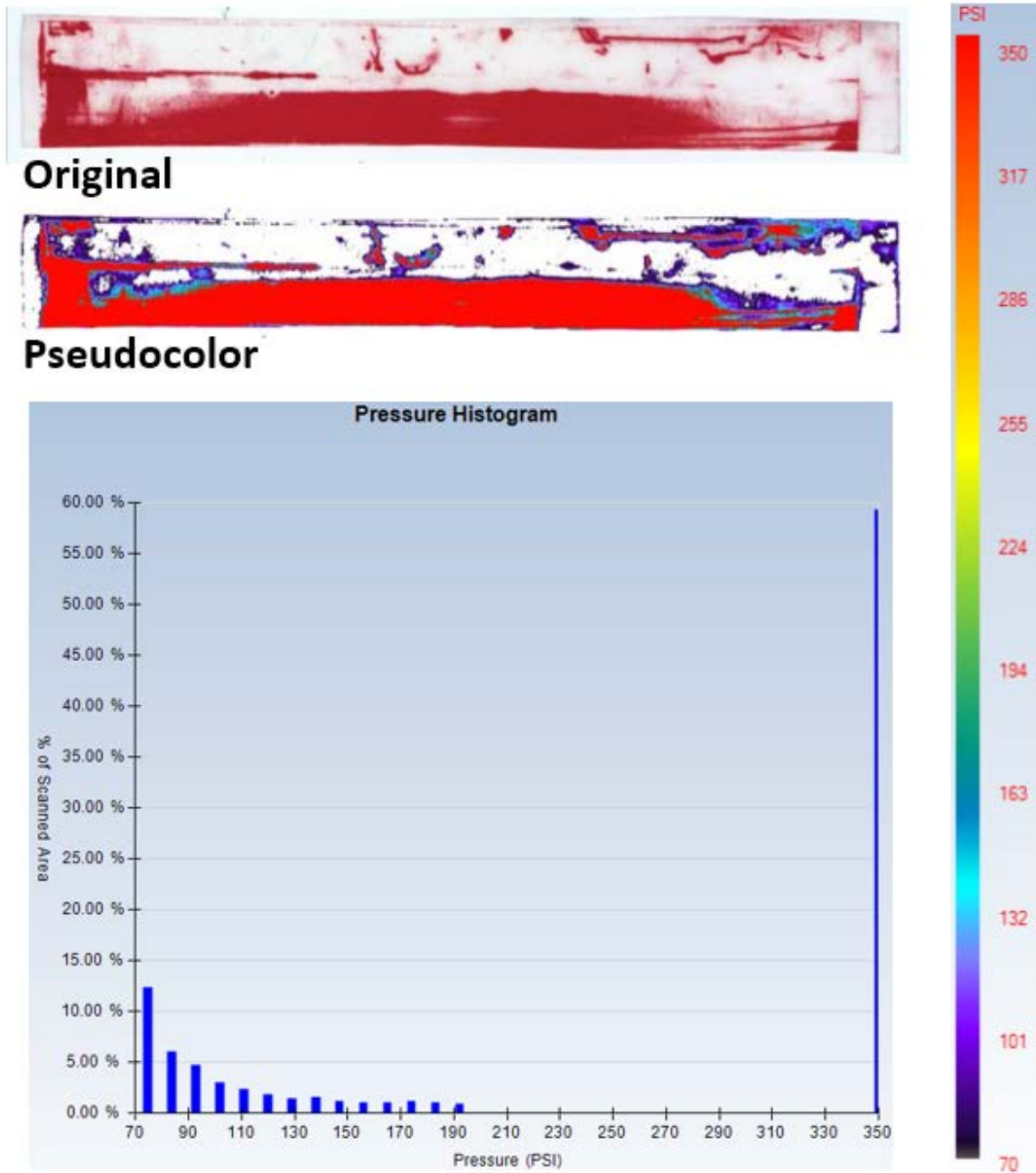
Figure 58: Pressure Analysis with Superlow Film – DHU
