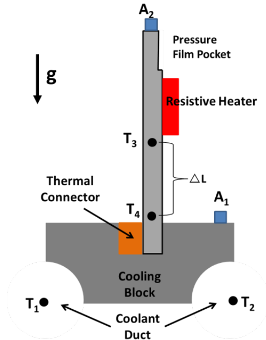
Figure A2: Schematic of Temperature Monitoring and Vibration Detection Setup for RevCon IV
