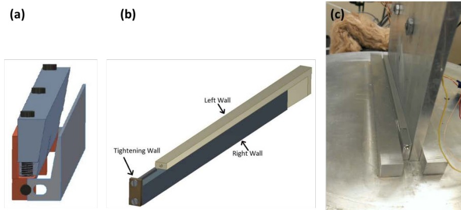
Figure 41: Another Two-piece Wedge Design Delivered by Ozyegin University Images are adopted from OU's report.
