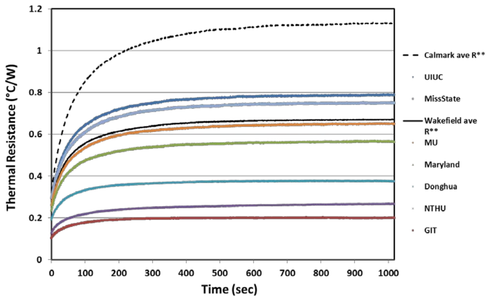
Figure 52: Comparison Thermal Resistance R^{**} from each Thermal Connector
