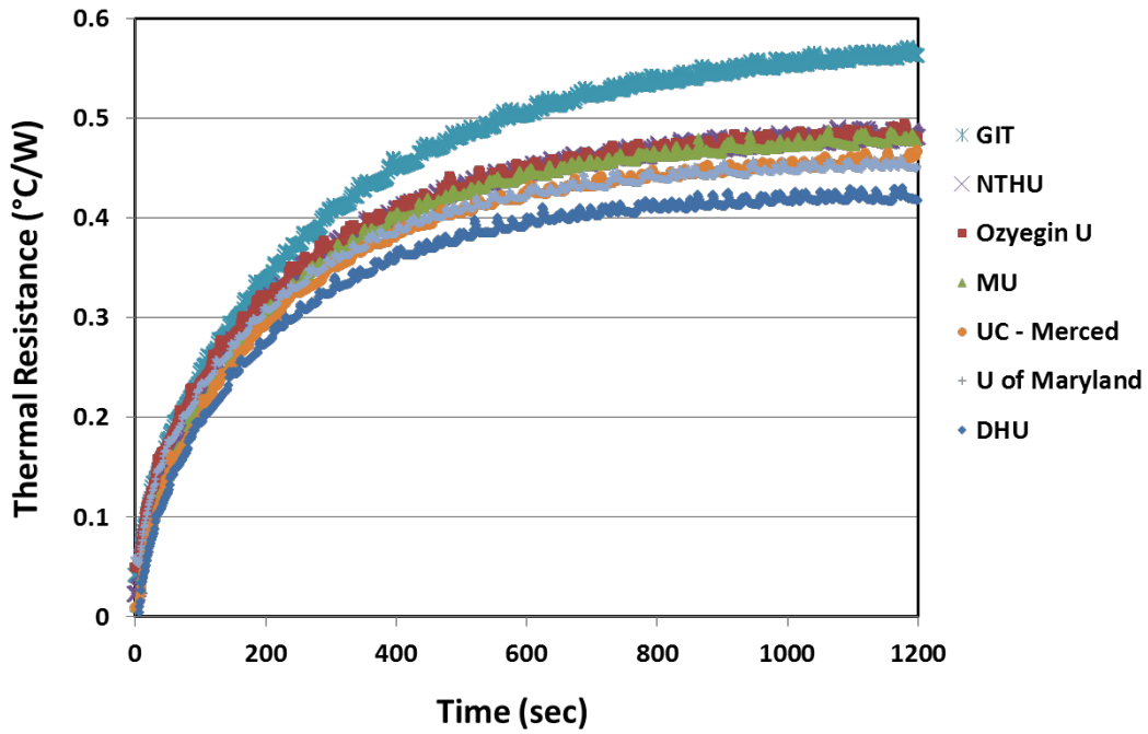
Figure 2: Comparison Thermal Resistance R from each Thermal Connector
