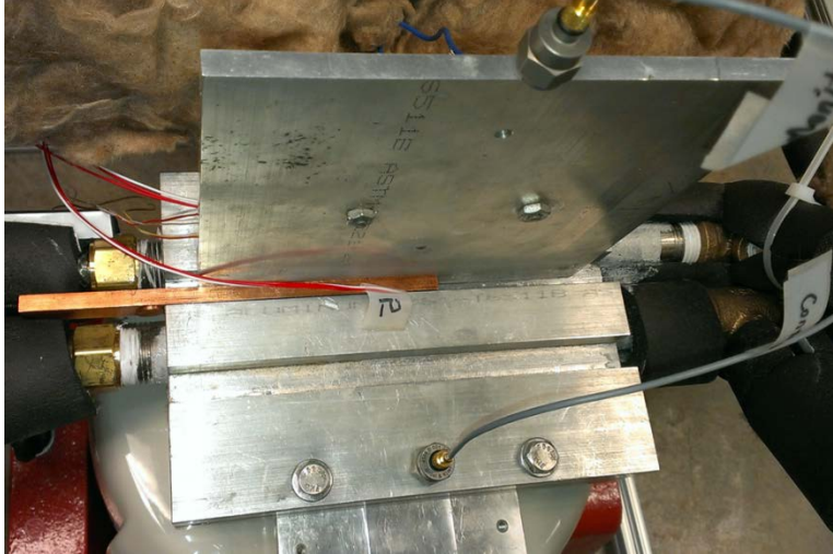
Figure 72: Hydraulic Thermal Connector Delivered by GIT
