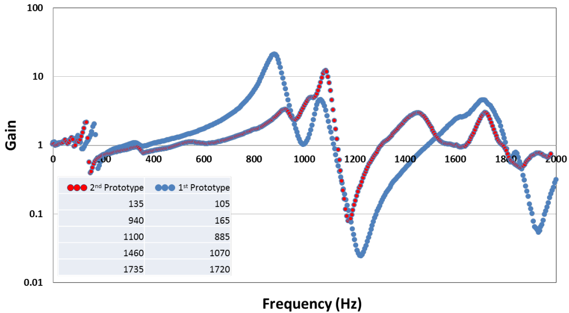
Figure 71: Frequency Response for DHU's Design
