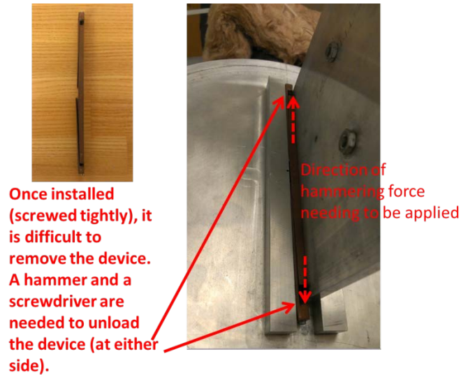
Figure 45: Thermal Connector Delivered by UCM
