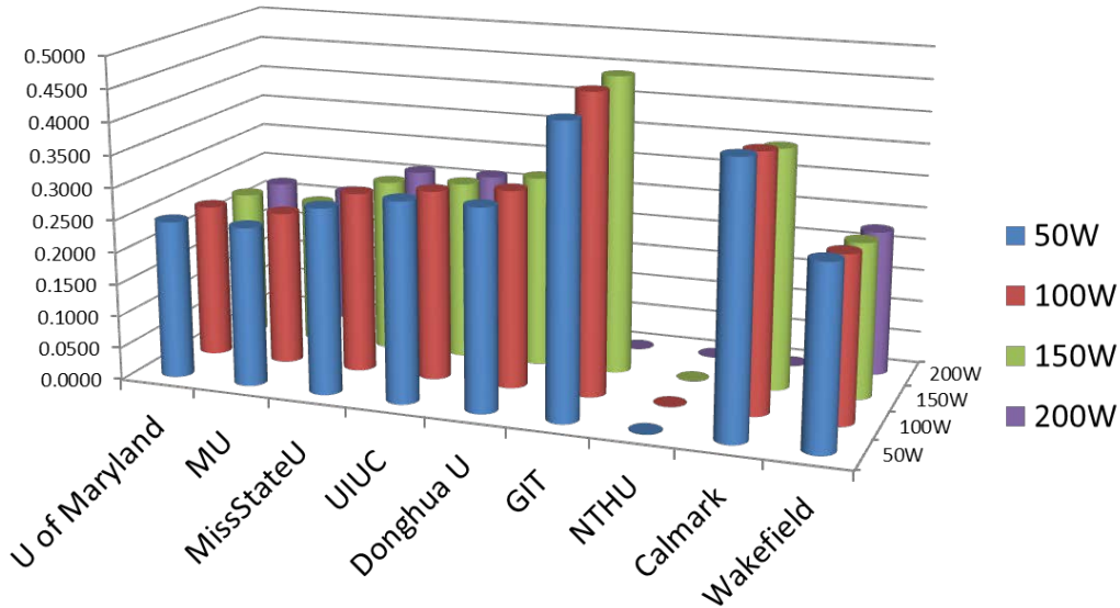
Figure 54: Comparison Chart of Thermal Resistance R* from each Thermal Connector
