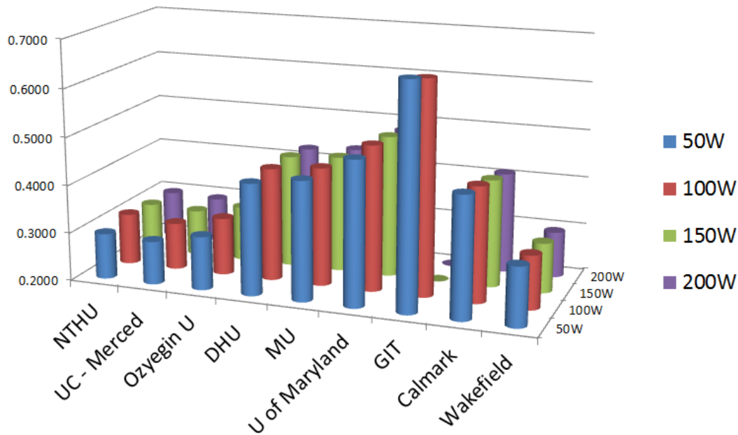
Figure 5: Comparison chart of Thermal Resistance R^* from each Thermal Connector
