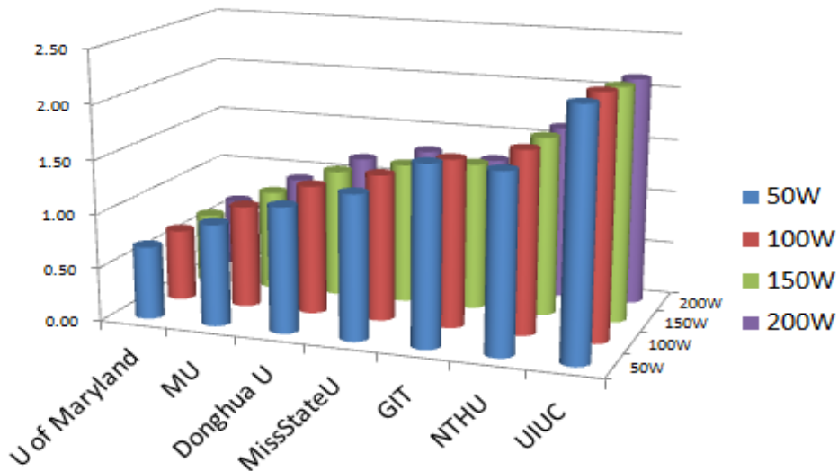
Figure 56: Comparison Chart of Thermal Resistance R* from each Thermal Connectors (1st prototype)
