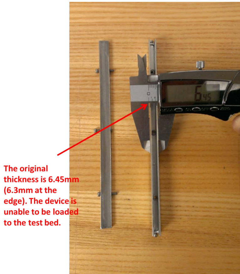
Figure 42: Up-down Wedge Design Delivered by Ozyegin University
