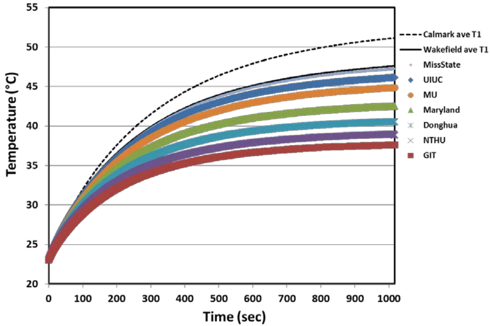
Figure 49: Comparison Temperature History of T_1 from each Thermal Connector Wakefield wedgelock (422C-480UMB in black solid line) and Calmark Card-lok (230-4.80H in black dotted line) are shown for comparison.
