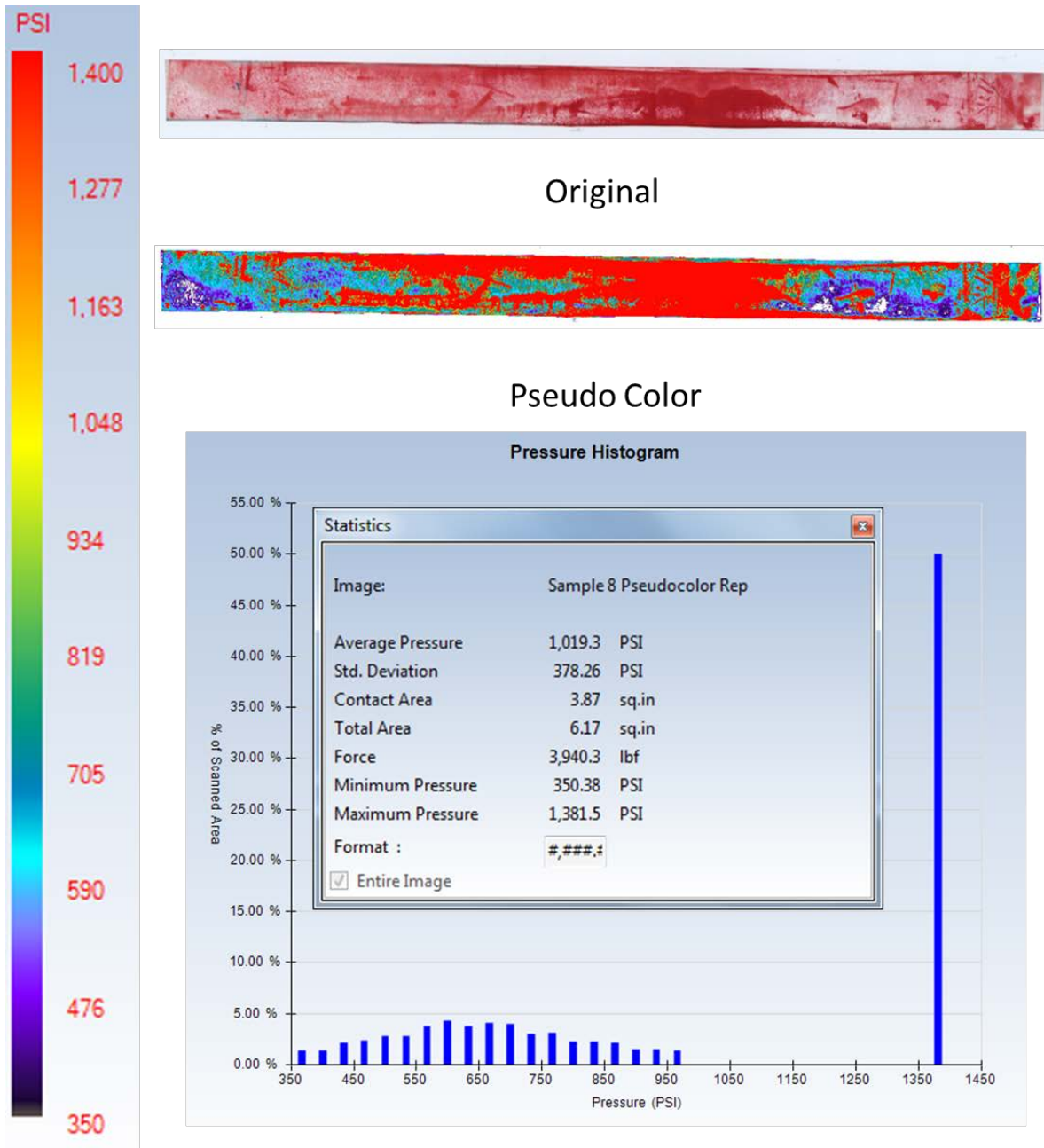
Figure 19: Pressure Analysis with Low Film – GIT
