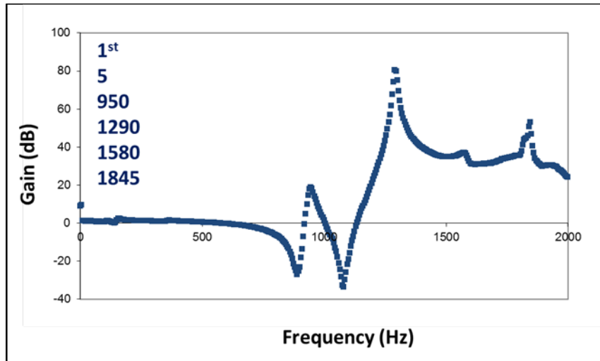
Figure 39: Frequency Response for Maryland's Design
