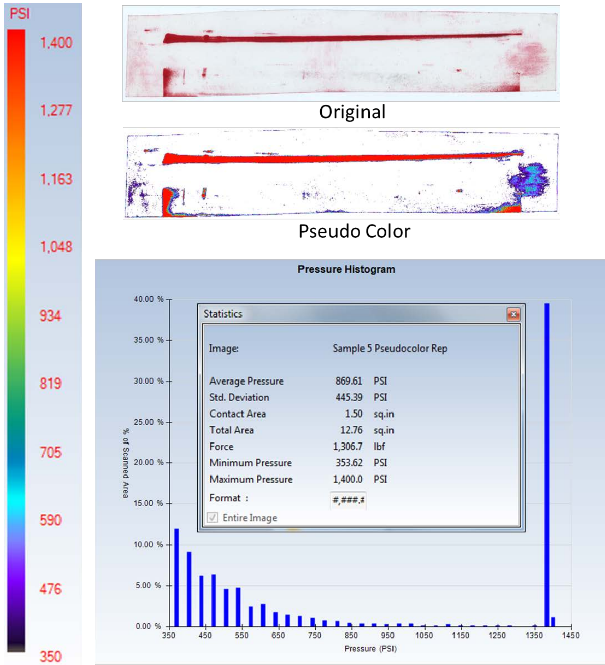
Figure 18: Pressure Analysis with Low Film – U of Baghdad
