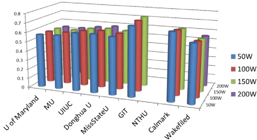
Figure 53: Comparison Chart of Thermal Resistance R from each Thermal Connectors
