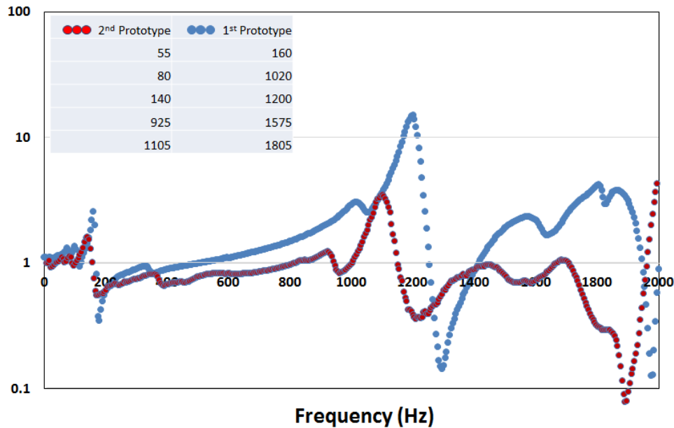
Figure 75: Frequency Response for MissStateU's Design
