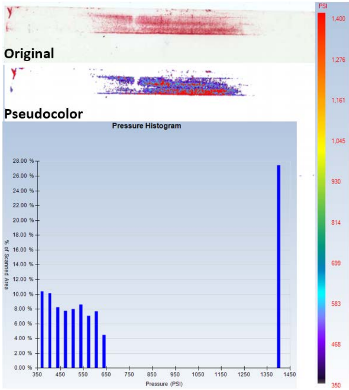
Figure 62: Pressure Analysis with Low Film – MU
