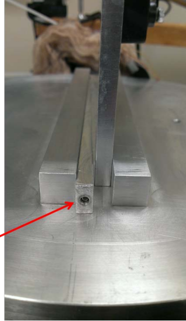
Figure 40: Two-wedge Thermal Connector Delivered by Maryland
