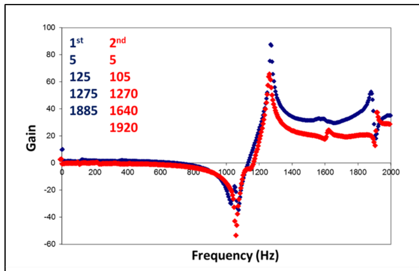
Figure 44: Frequency Response for UCM's Design
