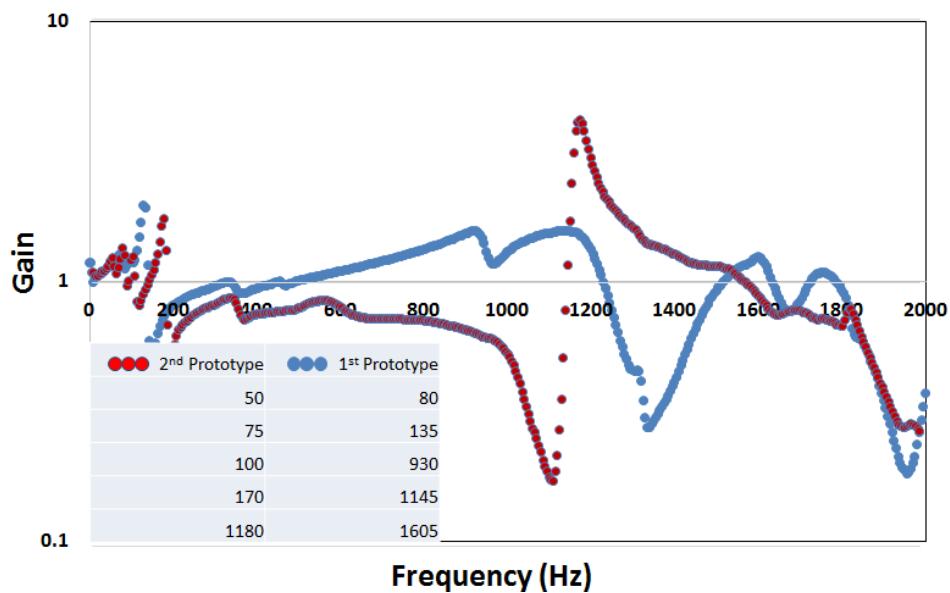
Figure 77: Frequency Response for MU's Design
