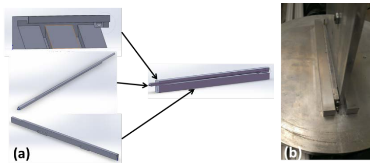
Figure 30: Three-wedge Design Delivered by MU Team
