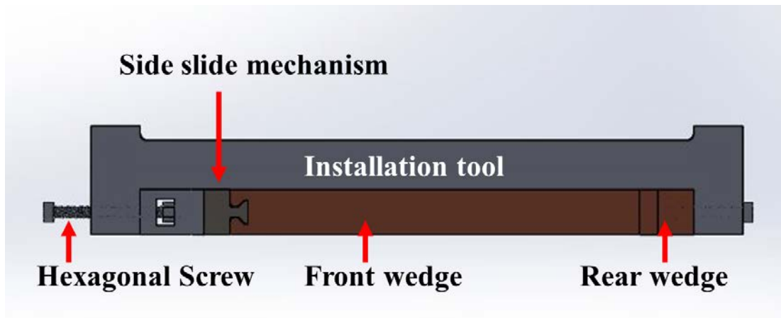
Figure 78: Side View of NTHU's Wedge Thermal Connector and its Auxiliary Tool for Loading and Unloading (Photo from NTHU report)
