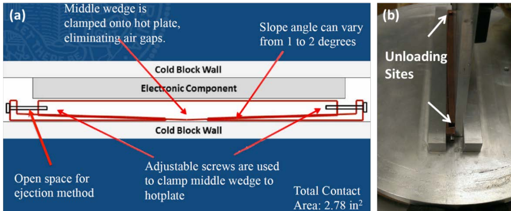
Figure 43: Three-wedge Thermal Connector Delivered by UCM
