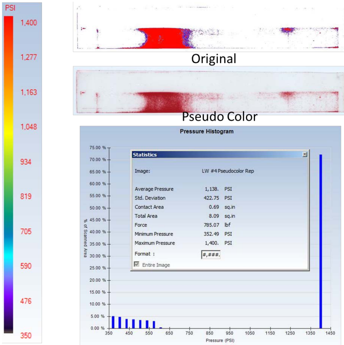
Figure 7: Pressure Analysis with Low Film – NTHU
