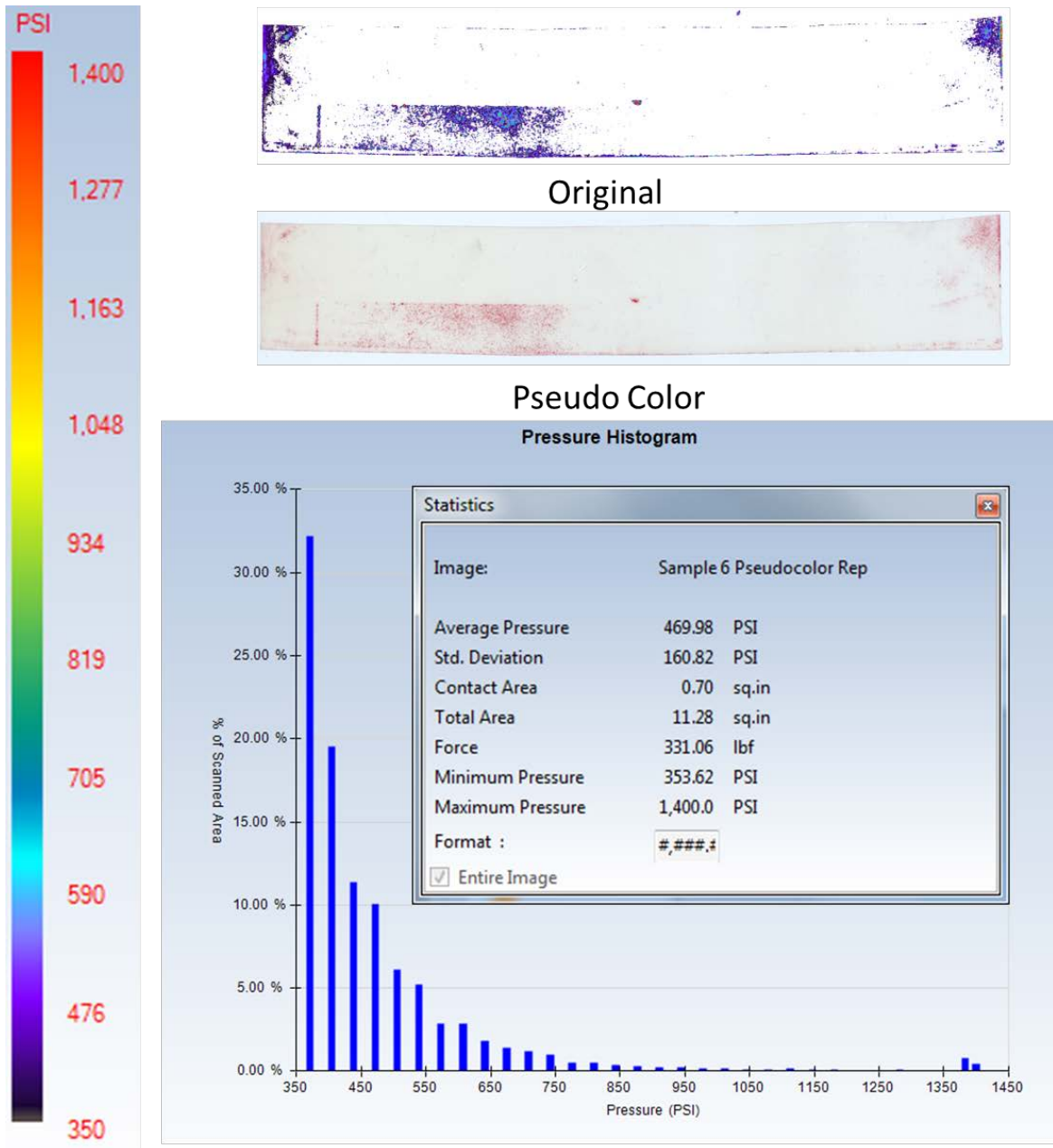
Figure 17: Pressure Analysis with Low Film – MU
