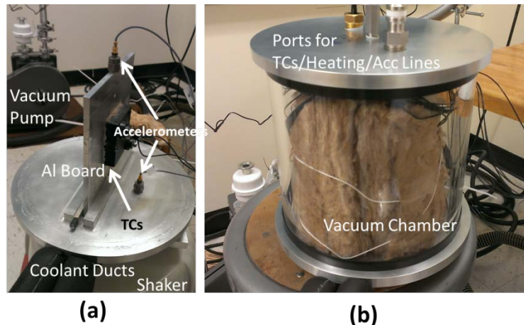
Figure A1: Testbed Assembly
