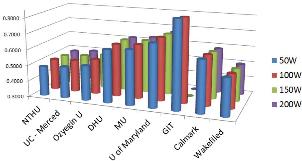
Figure 4: Comparison Chart of Thermal Resistance R from each Thermal Connector
