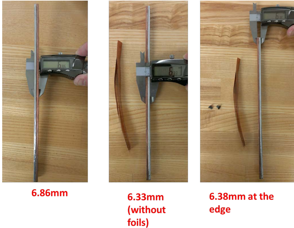
Figure 46: Sandwich Thermal Connector Designed by the University of Baghdad
