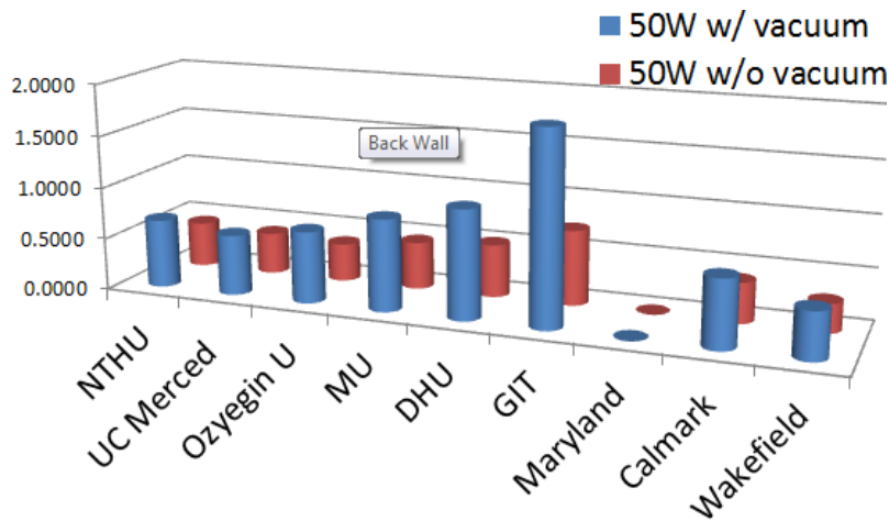
Figure 6: Comparison Chart of Thermal Resistance R from each Thermal Connector
