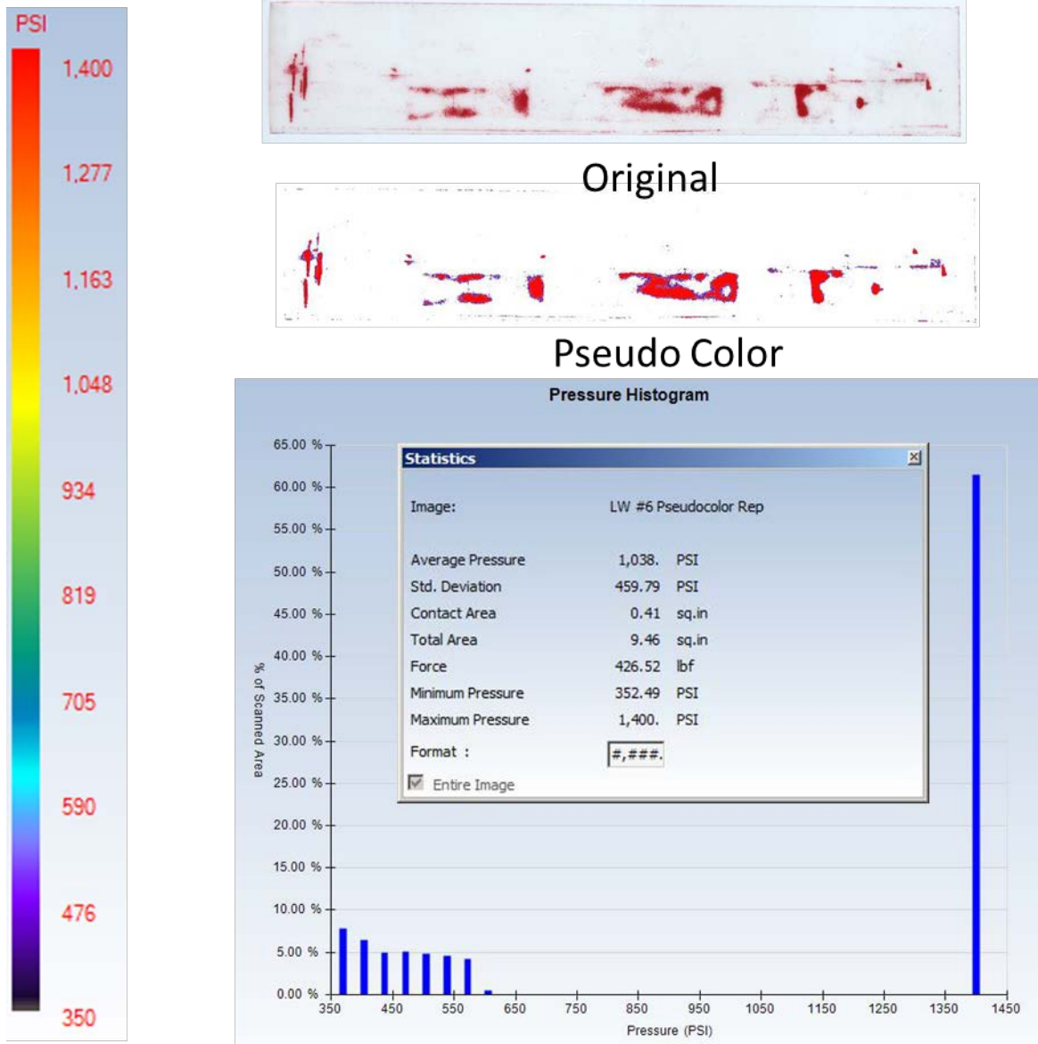
Figure 12: Pressure Analysis with Low Film – DHU
