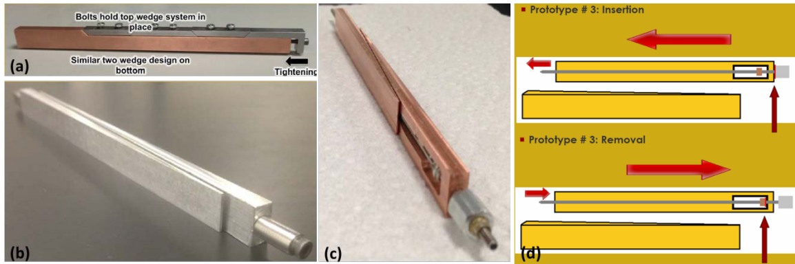
Figure 37: Evolution of Maryland's Prototypes
