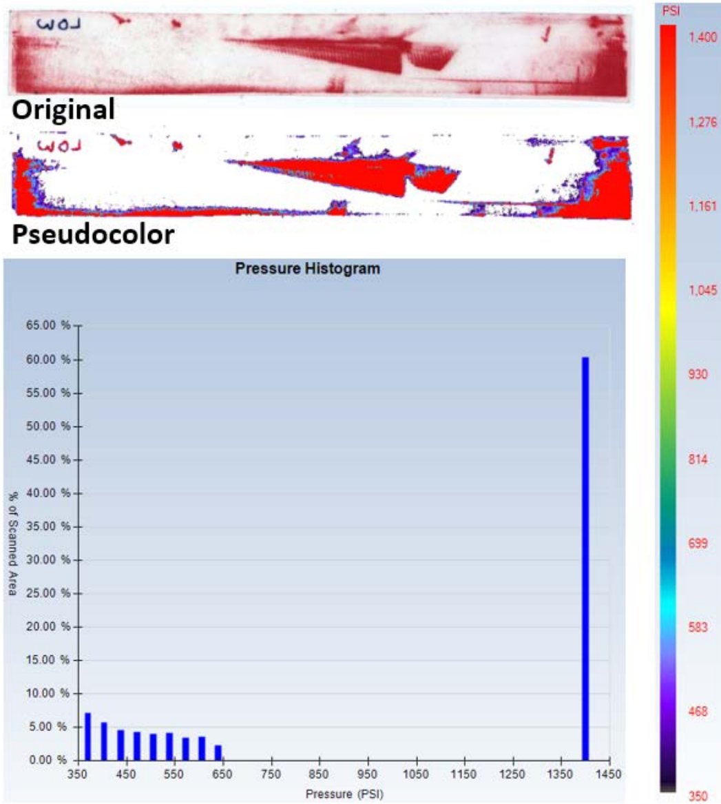
Figure 60: Pressure Analysis with Low Film – GIT
