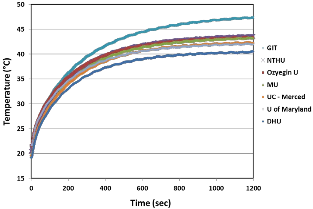
Figure 1: Comparison Temperature History of T 3 from each Thermal Connector
