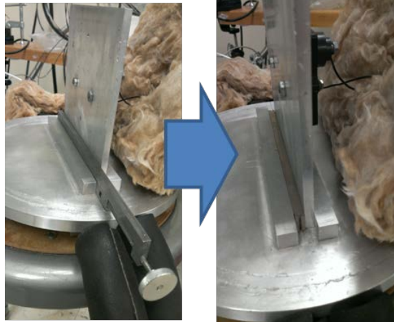
Figure 34: Side View of NTHU's Wedge Thermal Connector and its Auxiliary Tool for Loading and Unloading
