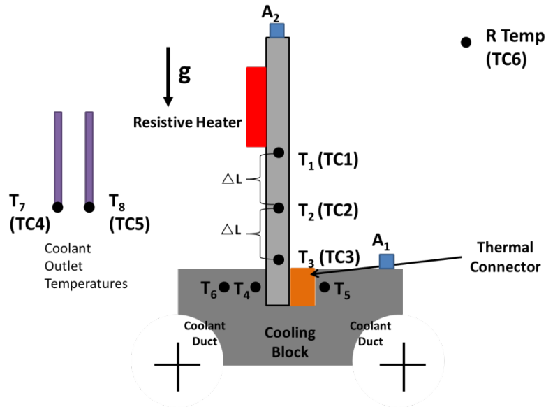
Figure A3: Schematic of Temperature Monitoring and Vibration Detection Setup for RevCon III
