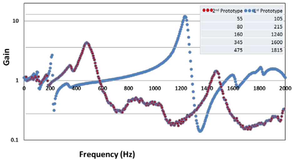
Figure 80: Frequency Response for UMD's Design
