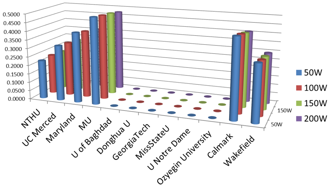
Figure 13: Comparison Chart of Thermal Resistance R from each Prototype, as well as Two Commercially Available Thermal Connectors
