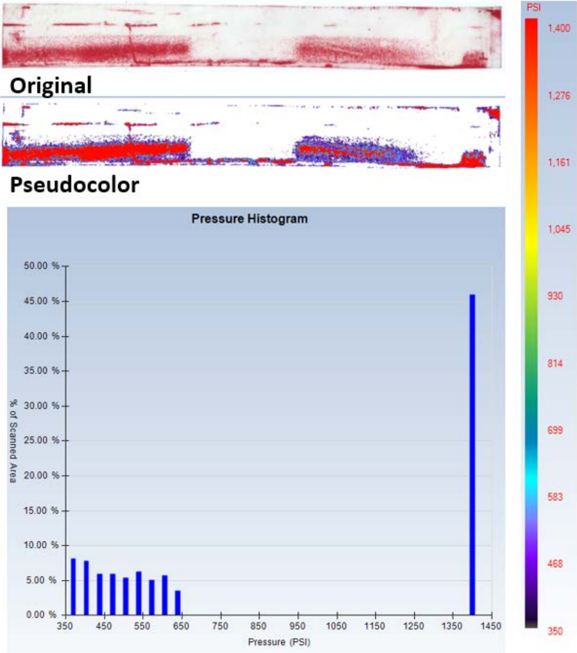
Figure 59: Pressure Analysis with Low Film – DHU
