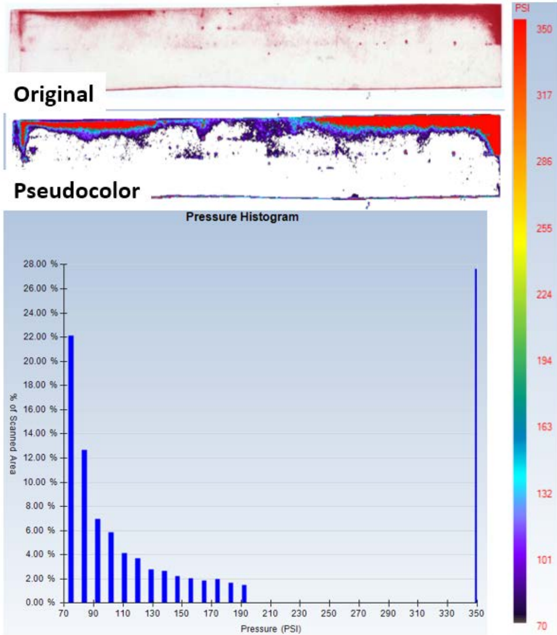
Figure 63: Pressure Analysis with Superlow film – NTHU
