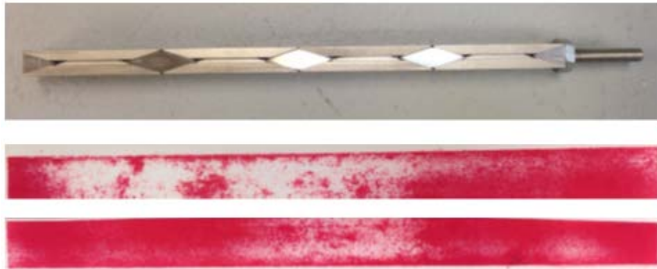
Figure 69: Pressure Distribution for Improved Double-sided Wedgelock, with Two Iterations
