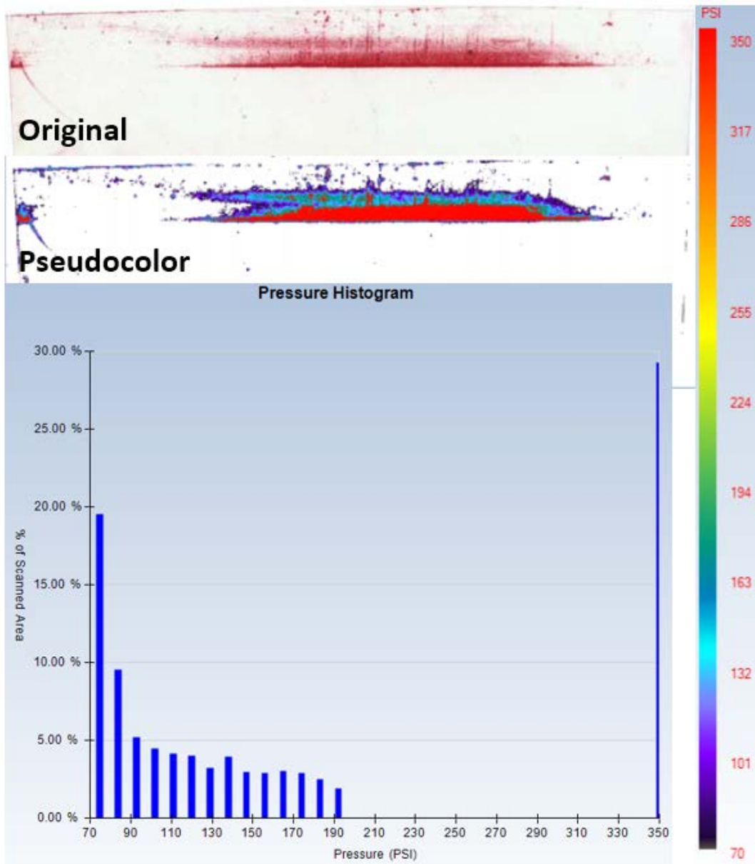
Figure 61: Pressure Analysis with Superlow Film – MU
