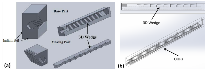
Figure 29: 3D Wedge Design Proposed by MU
