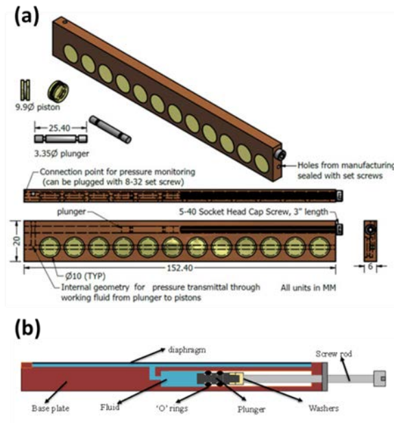
Figure 26: Thermo-hydraulic Design Proposed by GIT
