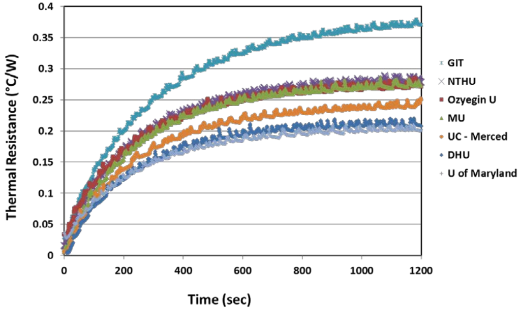
Figure 3: Comparison Thermal Resistance R^* from each Thermal Connector
