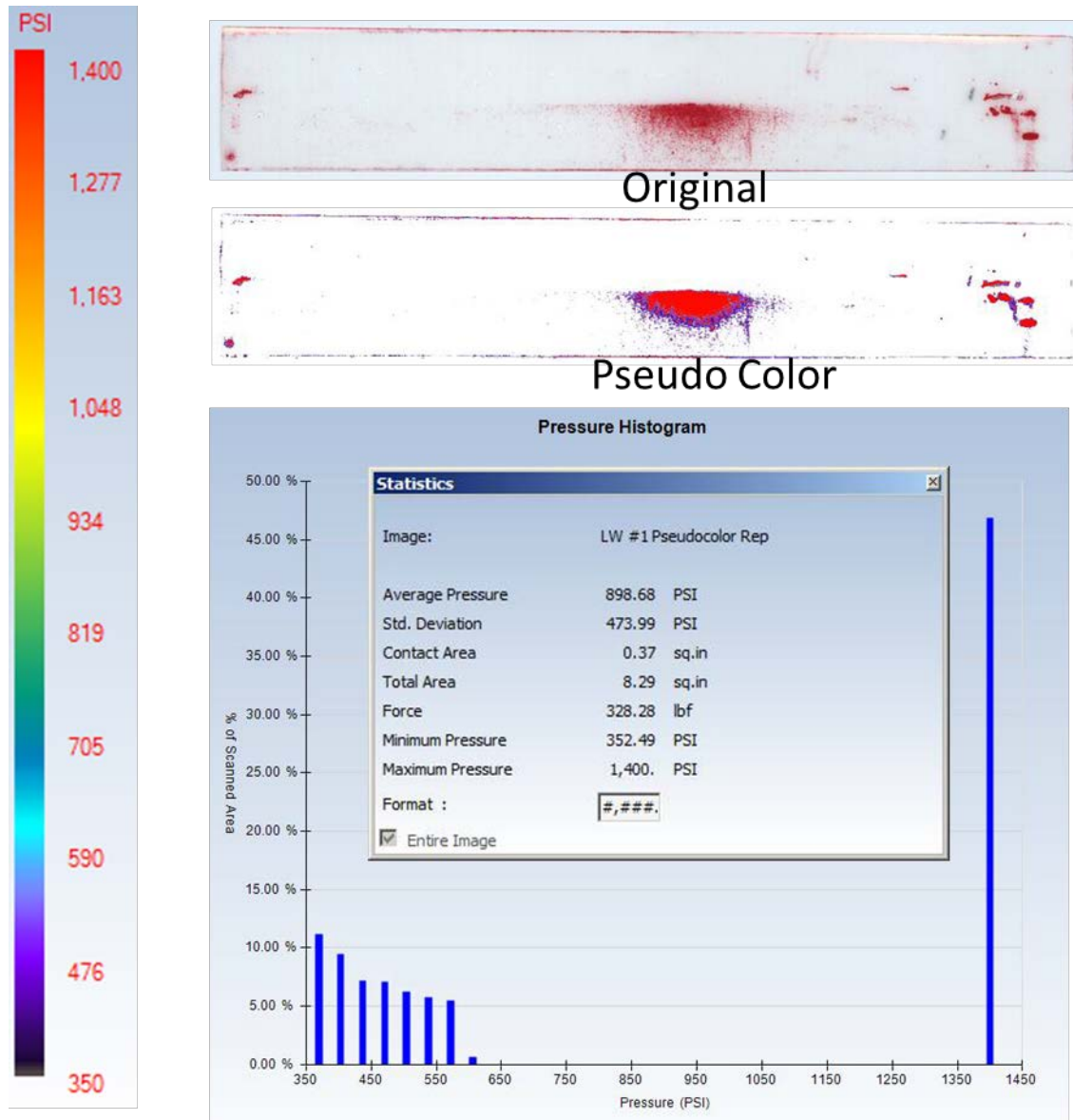
Figure 8: Pressure Analysis with Low Film – UC Merced
