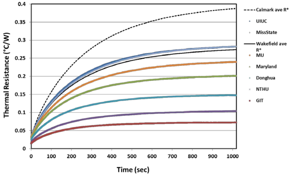
Figure 51: Comparison Thermal Resistance R^* from each Thermal Connector
