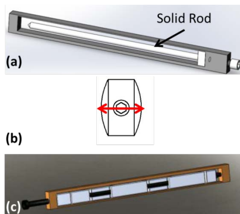
Figure 22: Concept of DHU's Thermal Connectors Images are adopted from DHU's report.
