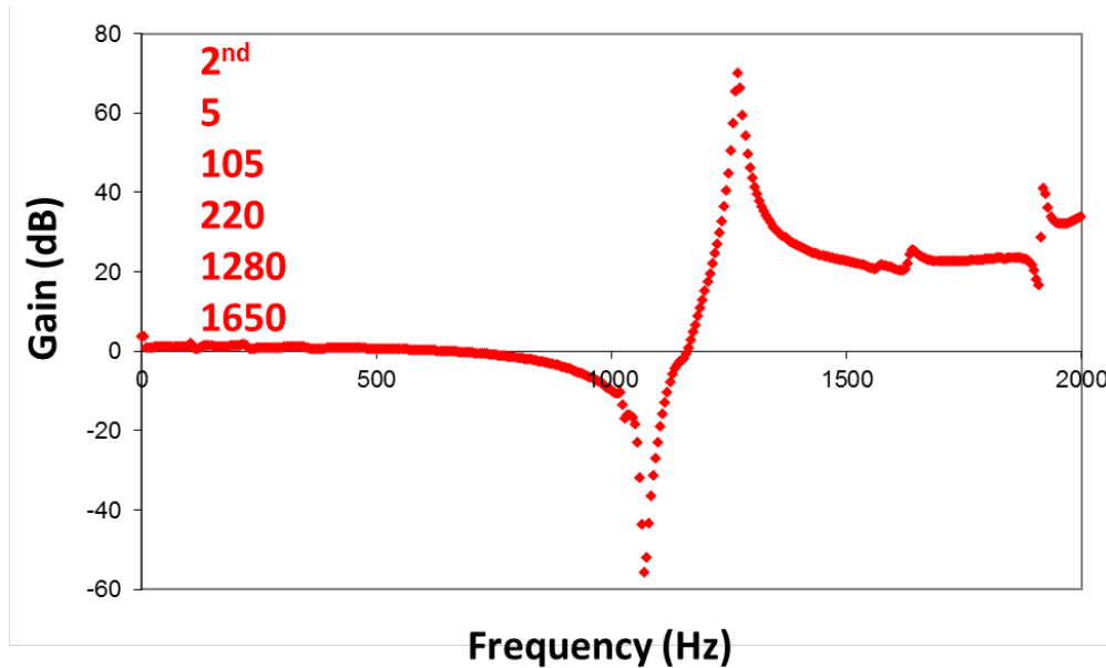
Figure 24: Frequency Response for Donghua University's Design
