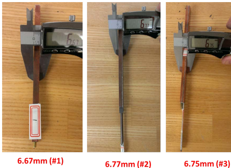
Figure 25: “Box” Thermal Connector Delivered by Donghua University
