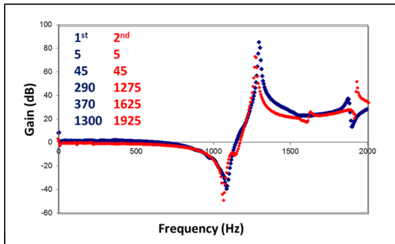
Figure 35: Frequency Response for NTHU's Design
