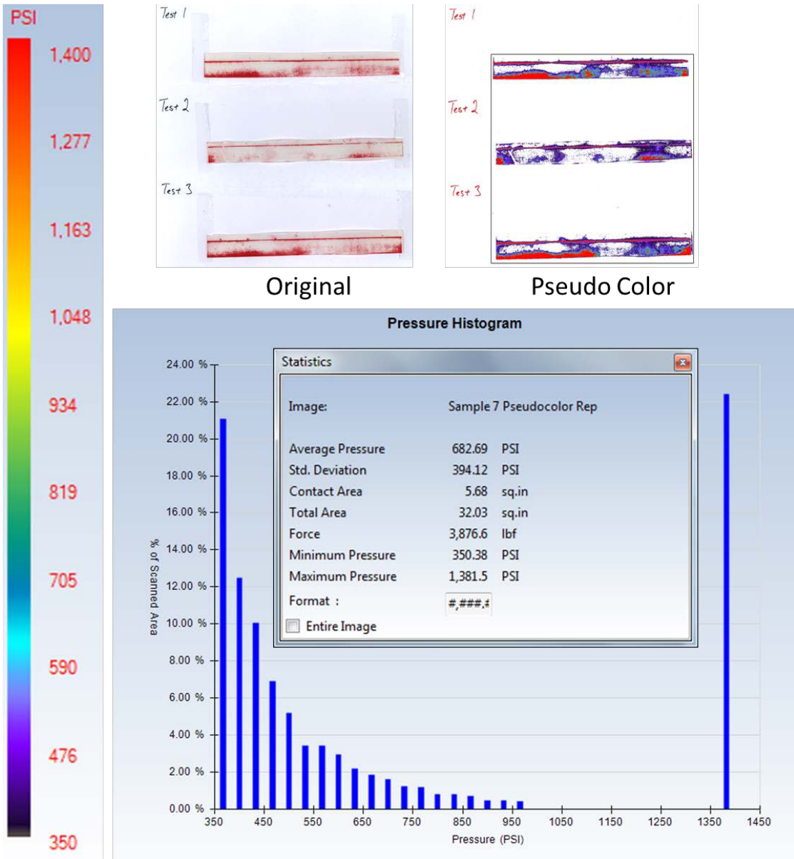
Figure 16: Pressure Analysis with Low Film – U of Maryland
