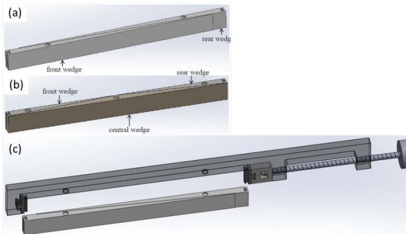
Figure 33: Wedge Design with Loading/Unloading Tool Proposed by NTHU (a) Two-wedge design, (b) three-wedge design, and (c) the tool provided to load/unload the device. Images are adopted from NTHU's report
