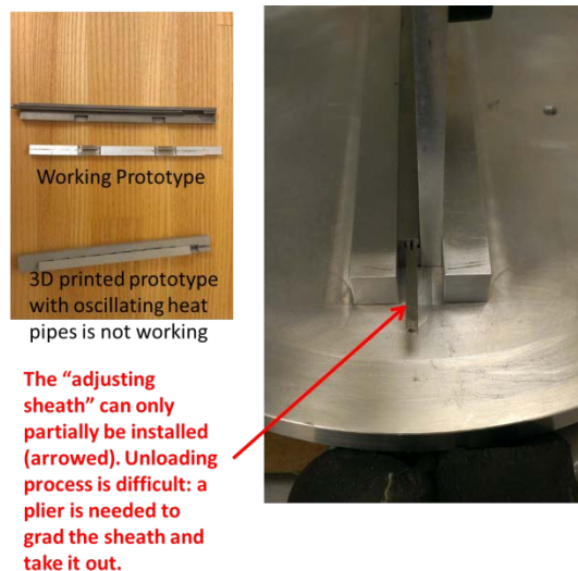
Figure 32: Thermal Connector Delivered by MU
