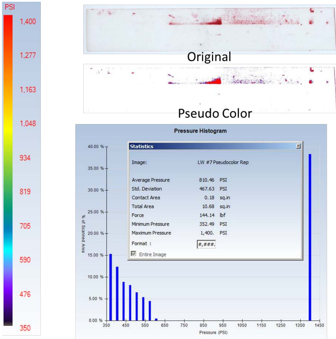
Figure 11: Pressure Analysis with Low Film – Ozyegin U
