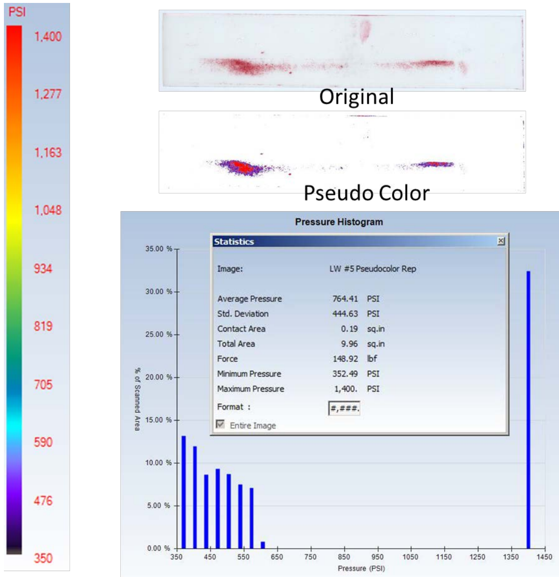
Figure 9: Pressure Analysis with Low Film – MU
