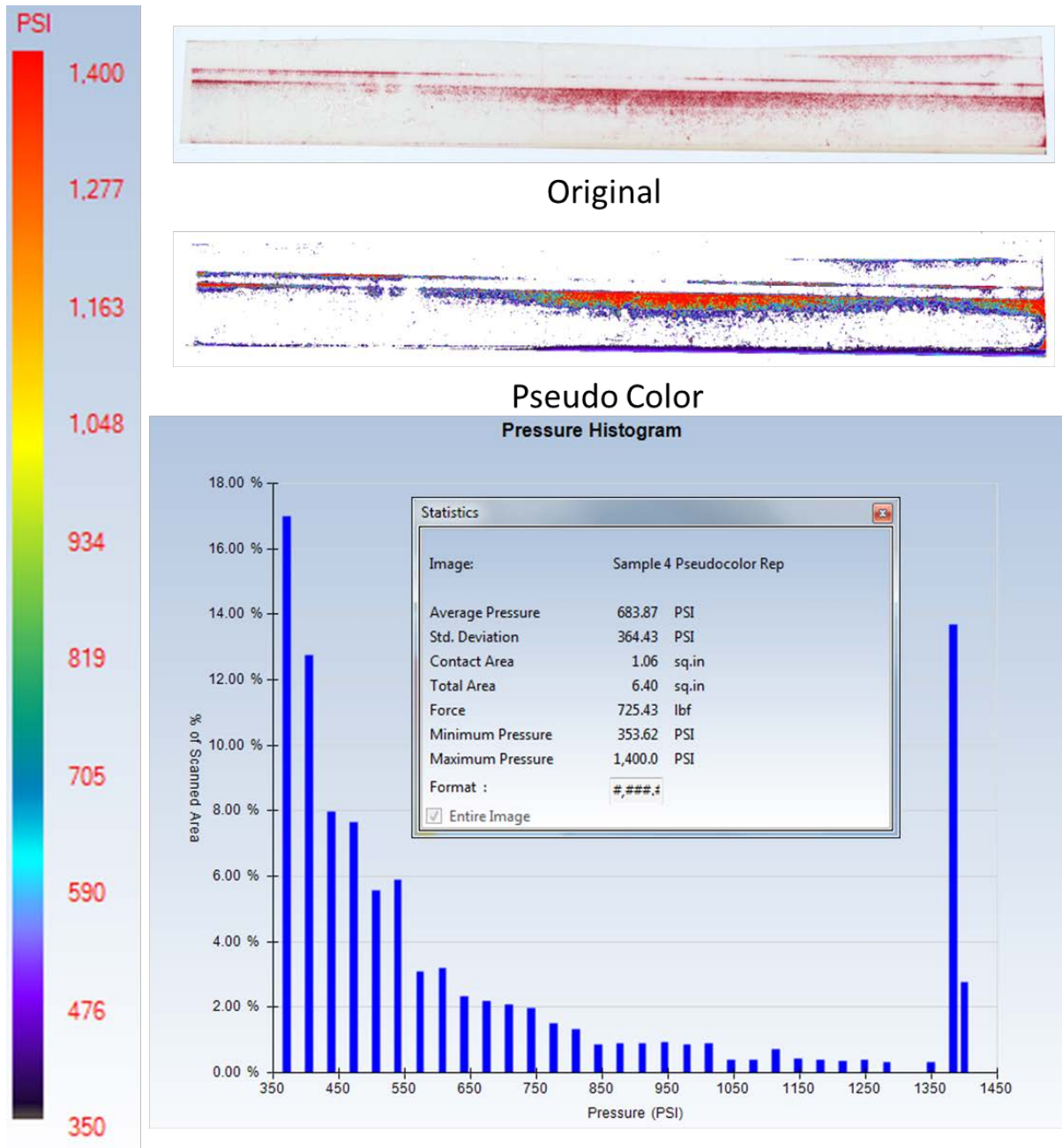
Figure 21: Pressure Analysis with Low Film – Ozyegin U
