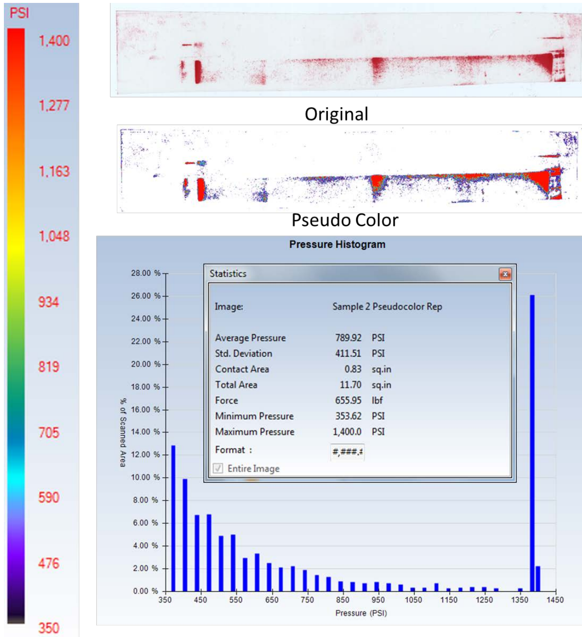
Figure 14: Pressure Analysis with Low Film – NTHU
