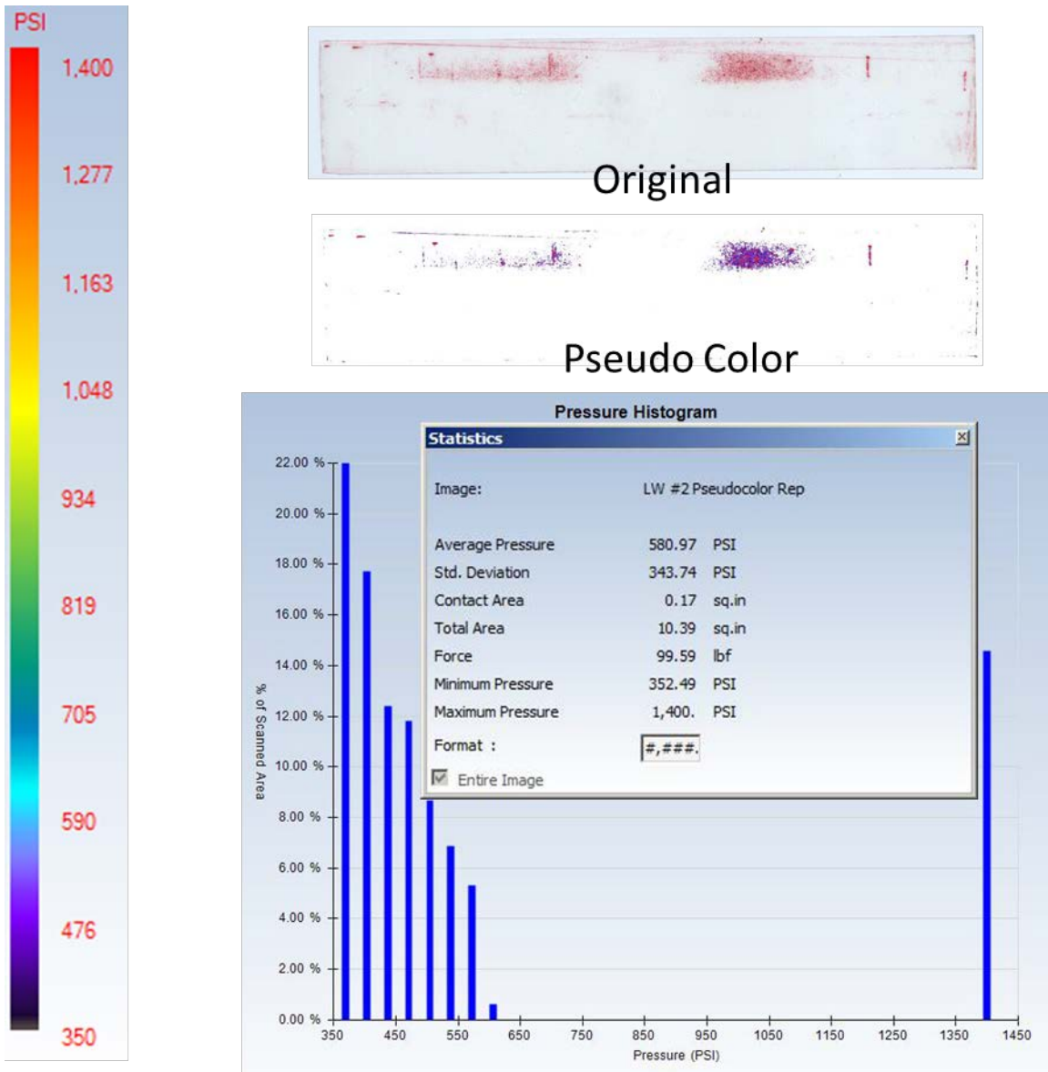
Figure 10: Pressure Analysis with Low Film – GIT
