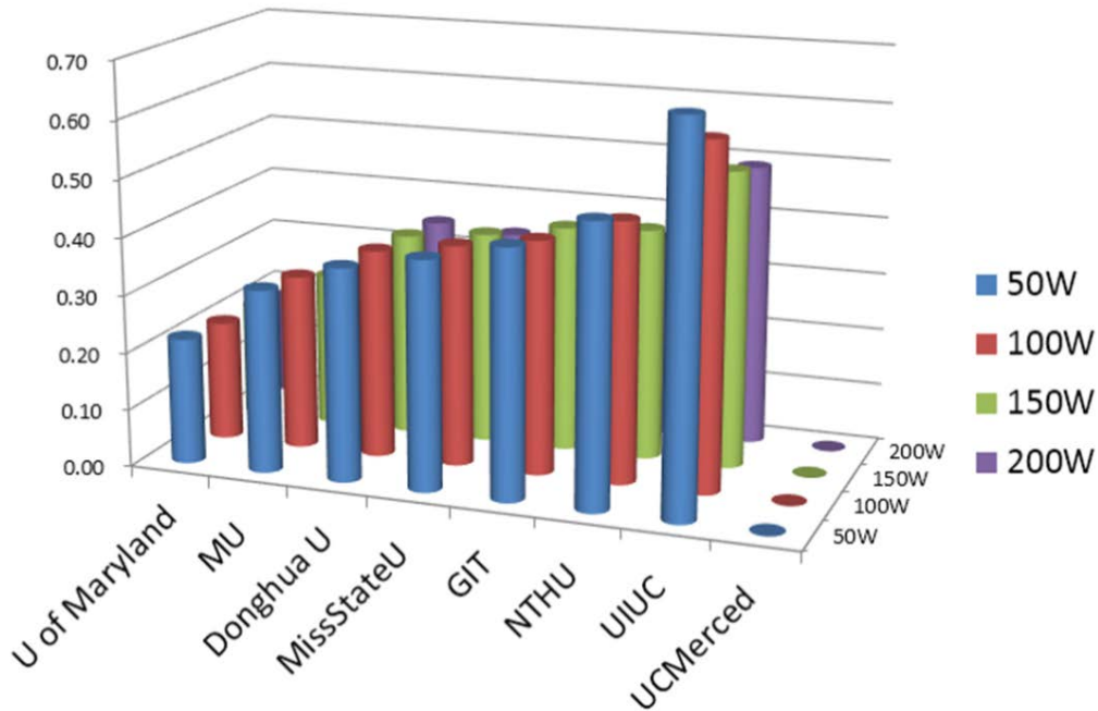
Figure 55: Comparison Chart of Thermal Resistance R from each Thermal Connector (1 st prototype)
