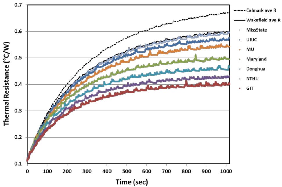
Figure 50: Comparison Thermal Resistance R from each Thermal Connector
