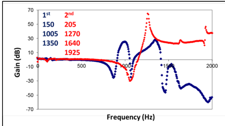
Figure 31: Frequency Response for MU's Design
