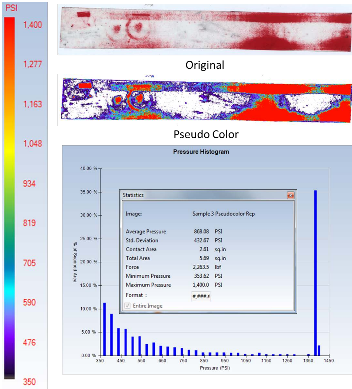
Figure 20: Pressure Analysis with Low Film – U of Notre Dame
