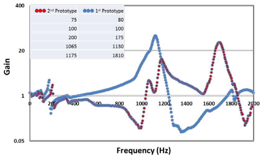
Figure 82: Frequency Response for UIUC's Design
