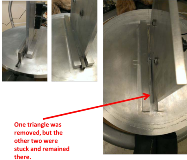
Figure 36: Three-wedge Thermal Connector Delivered from NTHU
