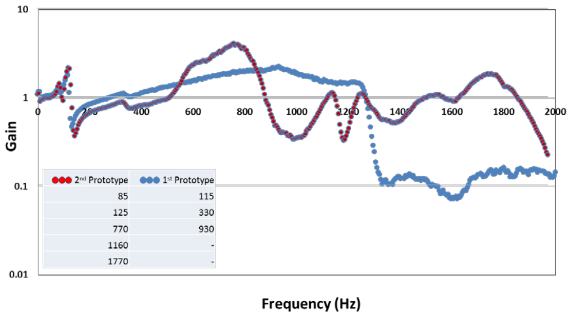
Figure 73: Frequency Response for GIT's Design
