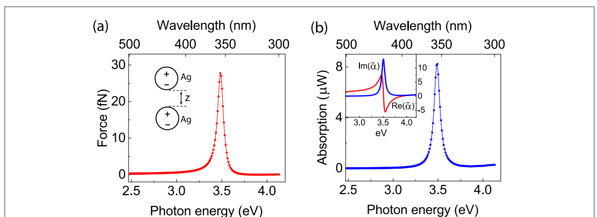
Figure 3. (a) Optical gradient force spectrum of two silver spheres with radius r = 10\text{ nm} separated by z = 20\text{ nm} subject to external optical field E = 10^6\text{ V m}^{-1} . (b) Absorption spectrum of the two spheres with symmetric resonance at 3.5\text{ eV} . Inset: real and imaginary part of the normalized polarizability \bar{\alpha} = (\epsilon_{\text{Ag}} - 1)/(\epsilon_{\text{Ag}} + 2) for a silver sphere. Force and absorption spectra follow the imaginary part of \bar{\alpha}(\omega) .
