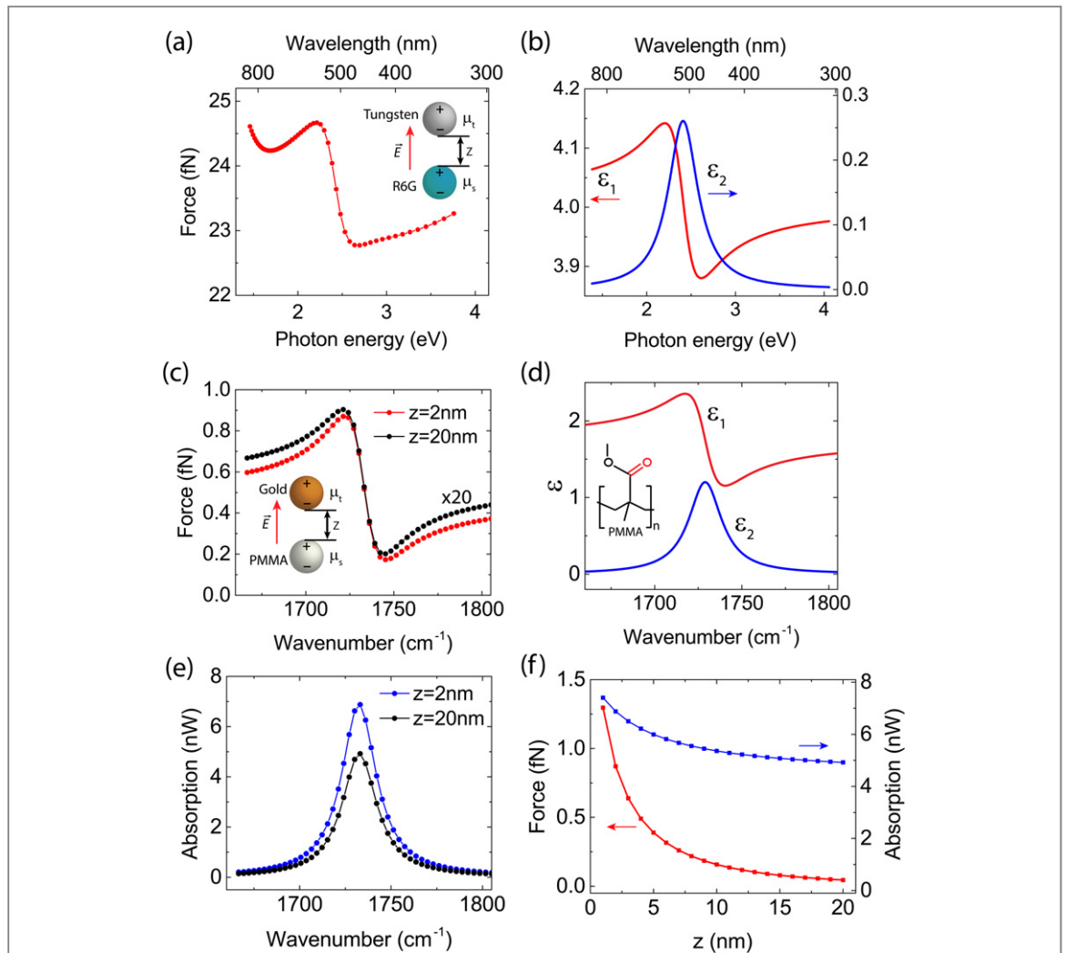
Figure 2. (a) Electronic resonant force spectrum between a tungsten tip and R6G sample (both of radius r = 10\text{ nm} ) subject to an optical field E = 10^6\text{ V m}^{-1} , separated by z = 2\text{ nm} . (b) Dielectric function of R6G \epsilon(\omega) = \epsilon_1(\omega) + i\epsilon_2(\omega) modeled as a single harmonic oscillator. (c) Corresponding force spectra between a gold sphere and PMMA sample of radii r = 10\text{ nm} . Dispersive force spectrum at separation distance z = 20\text{ nm} (multiplied by 20, black) compared to force spectrum at z = 2\text{ nm} (red). (d) Dielectric function of PMMA \epsilon(\omega) = \epsilon_1(\omega) + i\epsilon_2(\omega) around the carbonyl resonance at 1729\text{ cm}^{-1} . (e) Simulated PMMA absorption at distances z = 20\text{ nm} (black) and z = 2\text{ nm} (blue). (f) The distance dependence of the optical force (red) on resonance shows a complex distance scaling, neither following a simple dipole-dipole power law nor exponential scaling. The slight increase of optical absorption (blue) is due to local field enhancement in the gap region.
