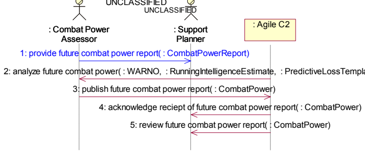
Determine Combat Power - SAUC03 Sequence Diagram Revised: 16 Jun 06 User Review: (Pending)
