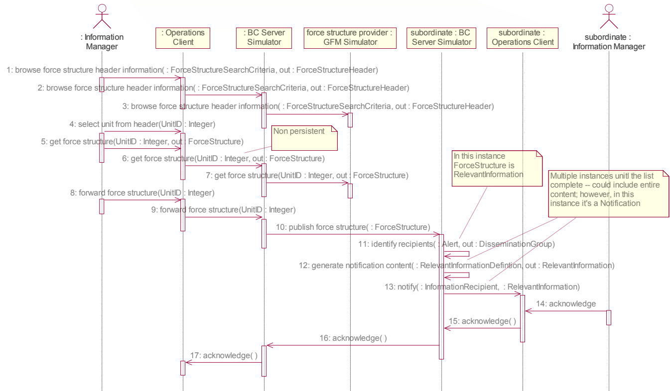
Populate Force Structure (SV-6) Physical Realization Diagram (Sequence Diagram) Revised: 08 Nov 2006 User Review: (Pending)
