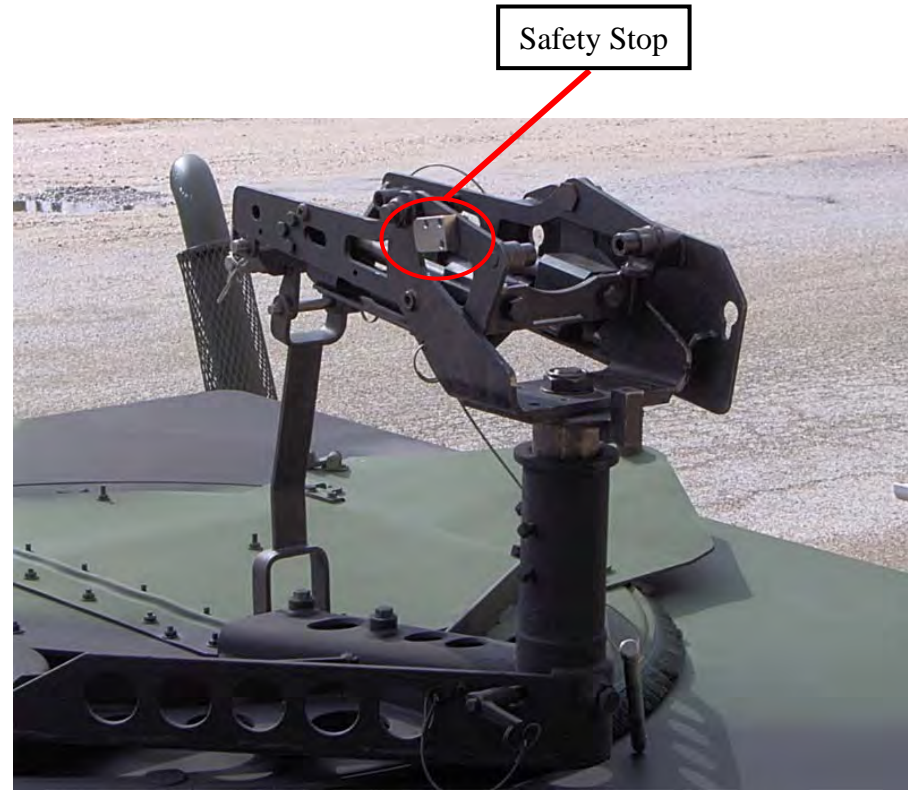
Mk 93 Pintle Installed on an A-MANPADS
