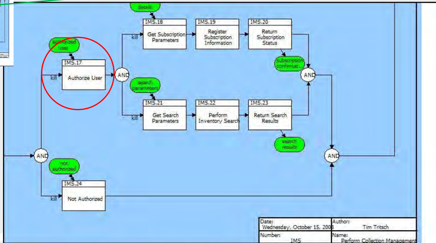
Management Enhanced FFBD
