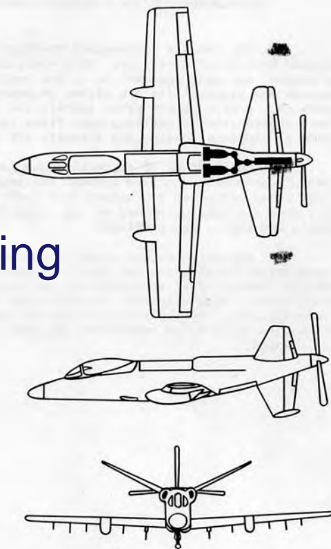
(U) NORTHROP RECOMMENDED-DESIGN GENERAL ARRANGEMENT (Figure UNCLASSIFIED)
