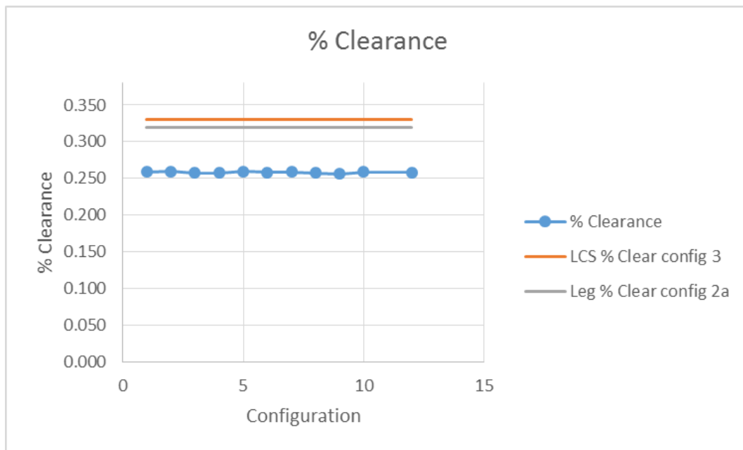
Figure 21. Mean of Percent Clearance vs. Configuration
