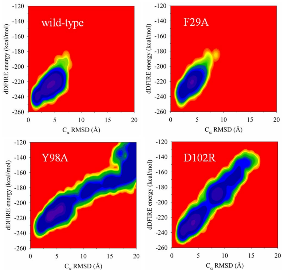
Figure 7. Two-dimensional population density profiles as a function of the statistical potential dDFIRE and C α RMSD from the starting crystallographic conformer B-chain at a temperature where the mutant Y98A is modeled to exhibit equal population between native and non-native states. Native-like states are defined as displacements from the starting structures by the approximation C α -RMSD < 5 Å. Comparisons are shown for the wild-type B-chain, F29A, Y98A and D102R. The color spectrum contains the extremes of blue for high population density and red for low density.
