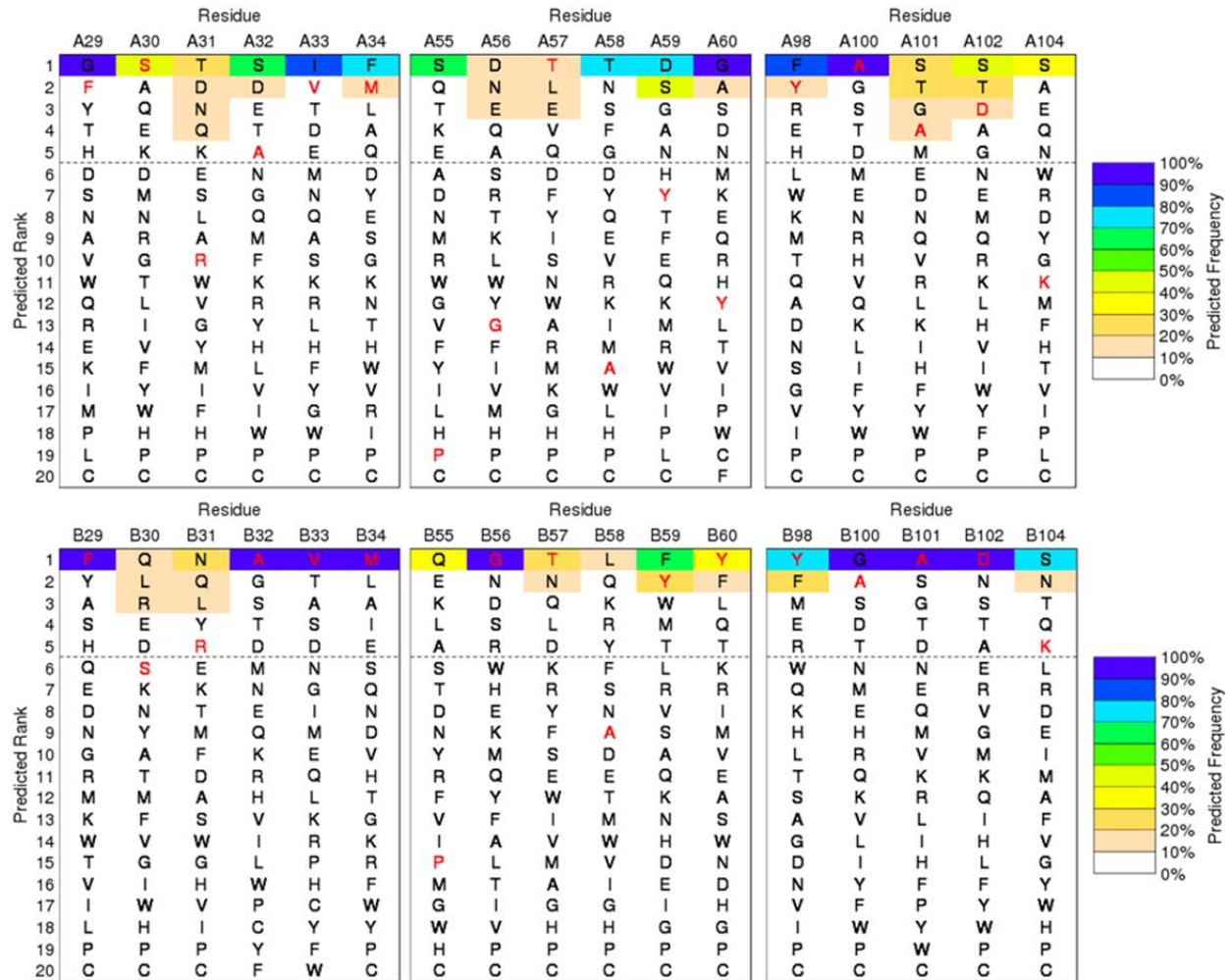
Figure 2. Selected sequence-tolerance profiles of the A-chain conformer (top graph) and B-chain conformer (bottom graph) determined by the RosettaBackrub method. Sequences colored red denote the wild-type residue. The color spectrum of each profile designates the predicted frequency of sequence-site placement along the A- or B-chain conformers. The horizontal line is arbitrarily positioned to highlight the five top-ranking sequences.
