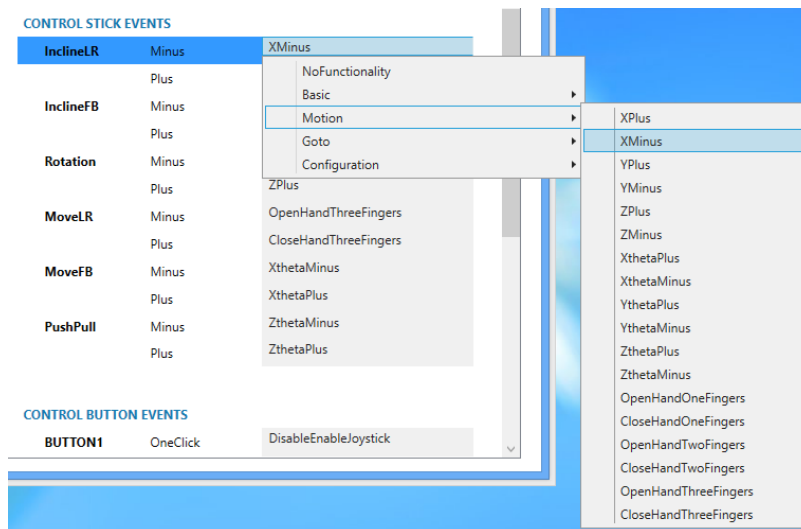
Figure 41. Associated functionality/motion.
