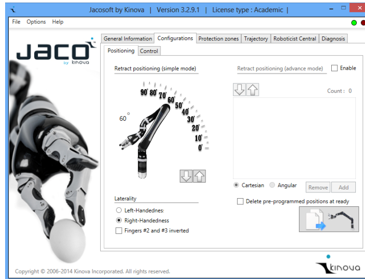
Figure 7. Configurations/Positioning tab.
