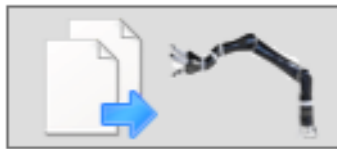
Figure 31. SEND button.
