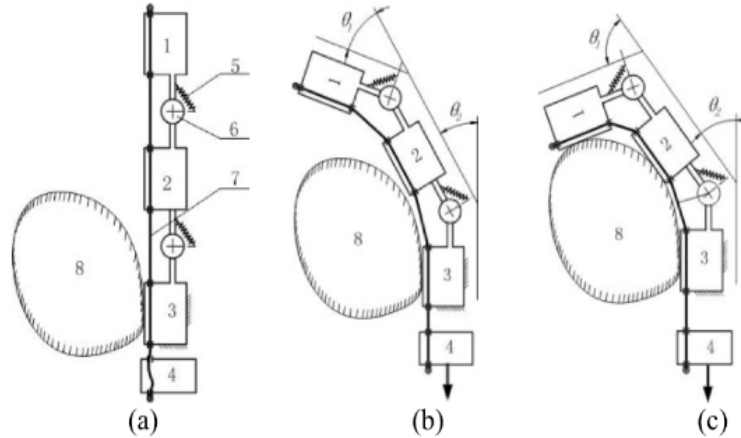
Figure 4. The three stages for grasping with an Underactuated Gripper.
