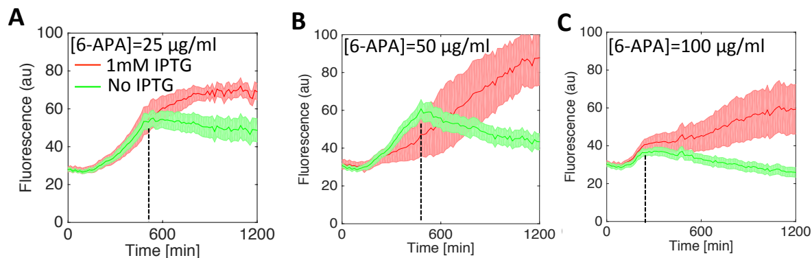
Figure 3. (A) 25 \mu\text{g}/\text{ml} (B) 50 \mu\text{g}/\text{ml} and (C) 100 \mu\text{g}/\text{ml} 6-APA was injected into droplets with (red) and without (green) 1mM IPTG rescuing. Black dash line indicates inflection point when the population stops growing without IPTG.
