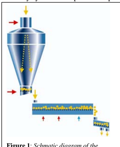
Figure 1: Schematic diagram of the principles of a small scale spray drier that can be used to convert fluid colloidal delivery systems into agglomerated powders (from Niro.com).
