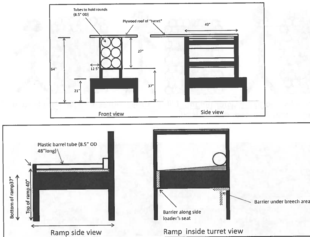
Figure 5. Diagrams and Photo of the Load Main Gun Simulation
