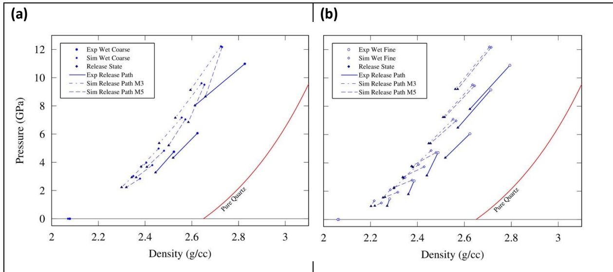
Figure 17. Experimental and simulated release paths (a) coarse grain sand (b) fine grain sand.
