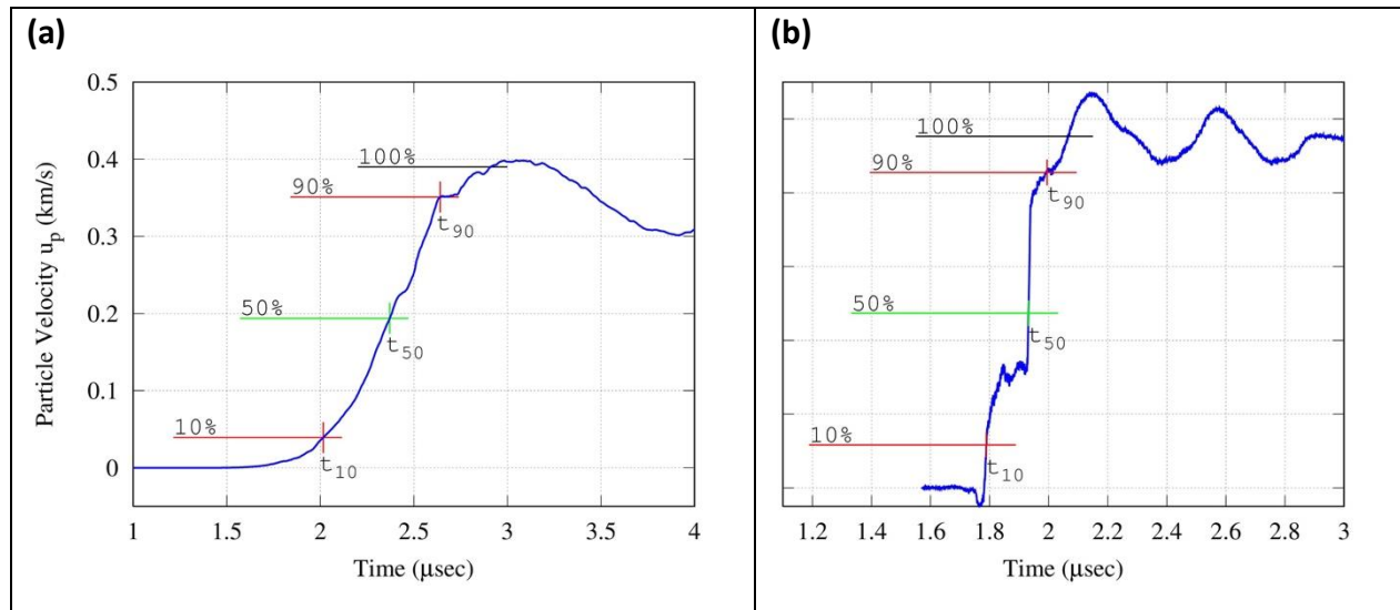
Figure 18. Particle velocity profiles depicting the location of 10%, 50%, 90%, and 100% of the particle velocity profile, u_p , and the corresponding times t_{10} , t_{50} , t_{90} . (a) CTH simulation u_0 = 500 m/s. (b) Experimental measurement using VISAR (h140) u_0 = 943 m/s. Both results are for dry, coarse sand.
