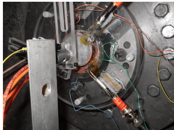
Figure 7. Photograph of sample mounted on GT 80mm gas gun along with diagnostics.
