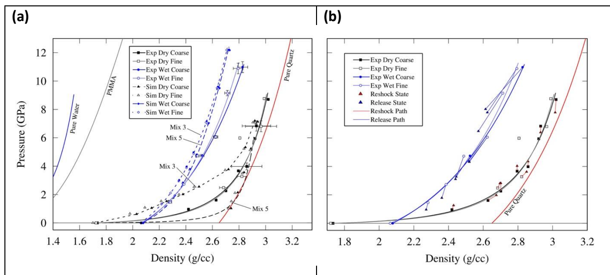
Figure 16. Pressure vs Density (a) experimental and simulated data (b) experimental data with reshock/release paths.
