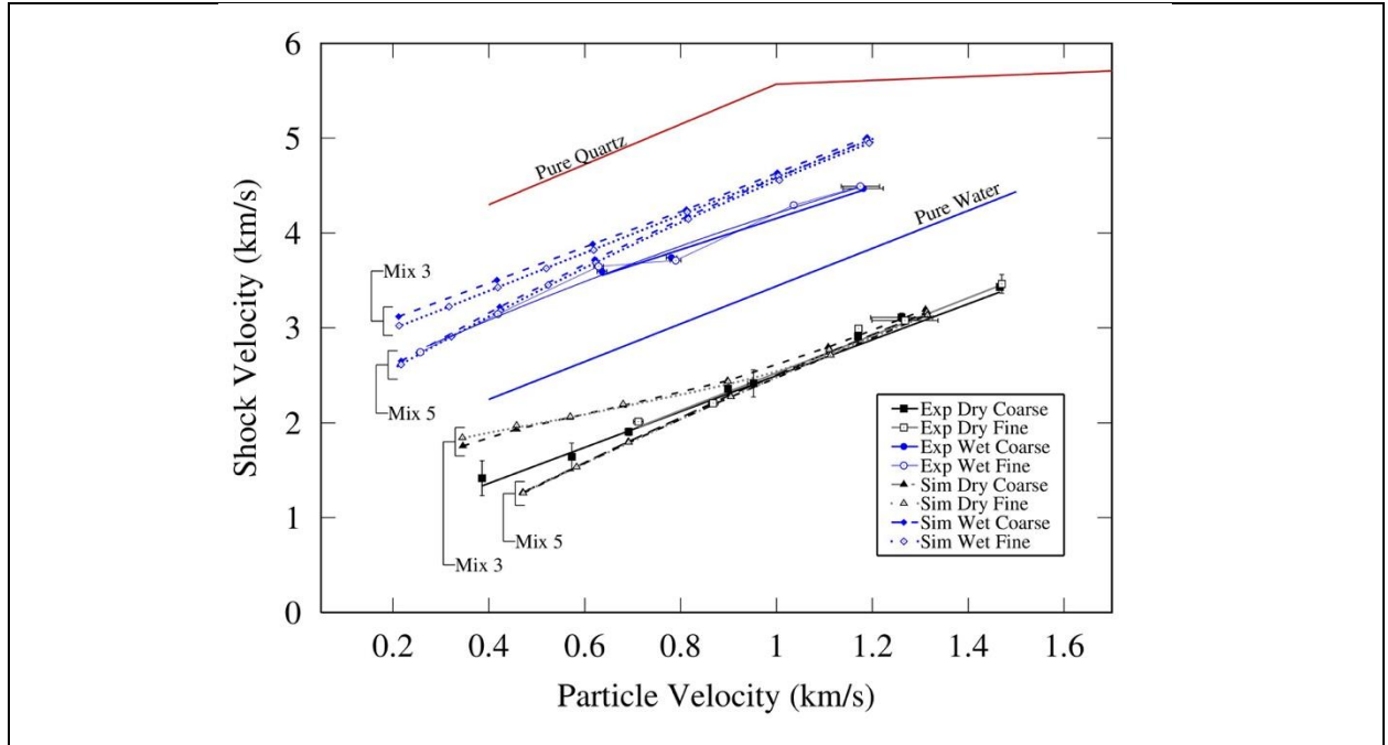
Figure 13. Simulated shock response compared to experimental data.
