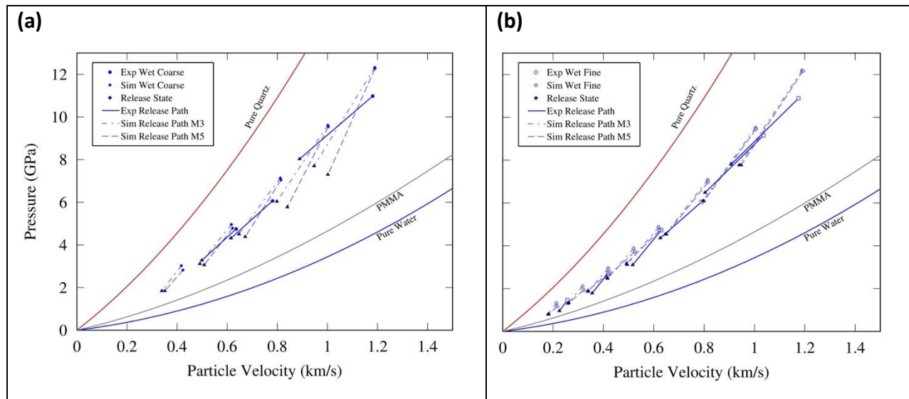
Figure 15. Experimental and simulated release paths (a) coarse grain sand (b) fine grain sand.
