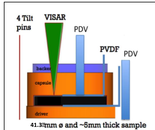
Figure 8. Schematic of modified capsule geometry used at AFRL.
