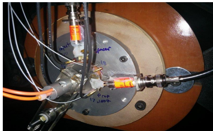
Figure 9. Photograph of the sample mounted to the AFRL Eglin target holding fixture.
