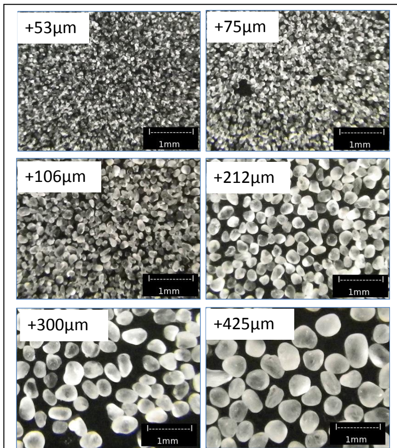
Figure 4. SEM images of various sieved particles of Oklahoma #1 pure sand.
