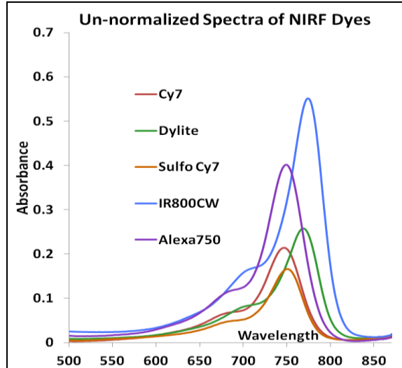
Fig. 4. Optical absorption spectra of five contrast agents. IRDye800CW (blue); AlexaFluor750 (purple); Cy7-NHS-ester (red); Cy7-sulfo (orange); Dylight800 (green).
