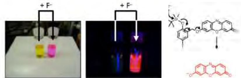
Released fluorophore provides a signal function
