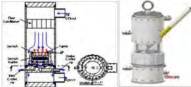
Fabric swatch test method: Chemical and Biological Agent Resistance Test (CBART)
