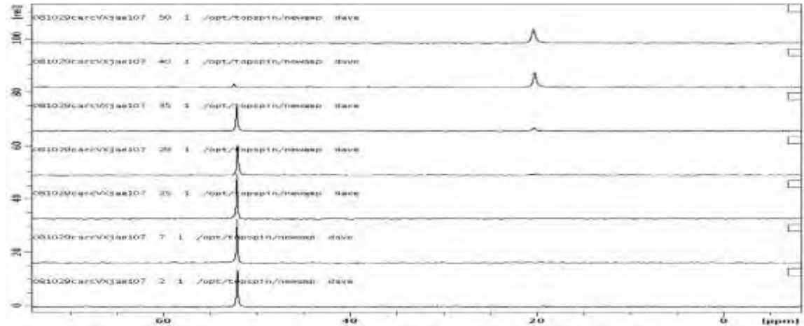
Solid-state NMR showing reaction of 1 \mu L VX to EMPA
