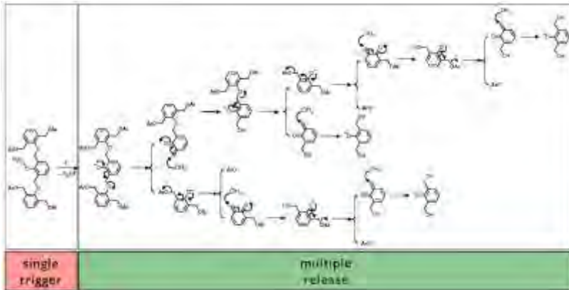
Triggered chain reactions act as molecular switches
