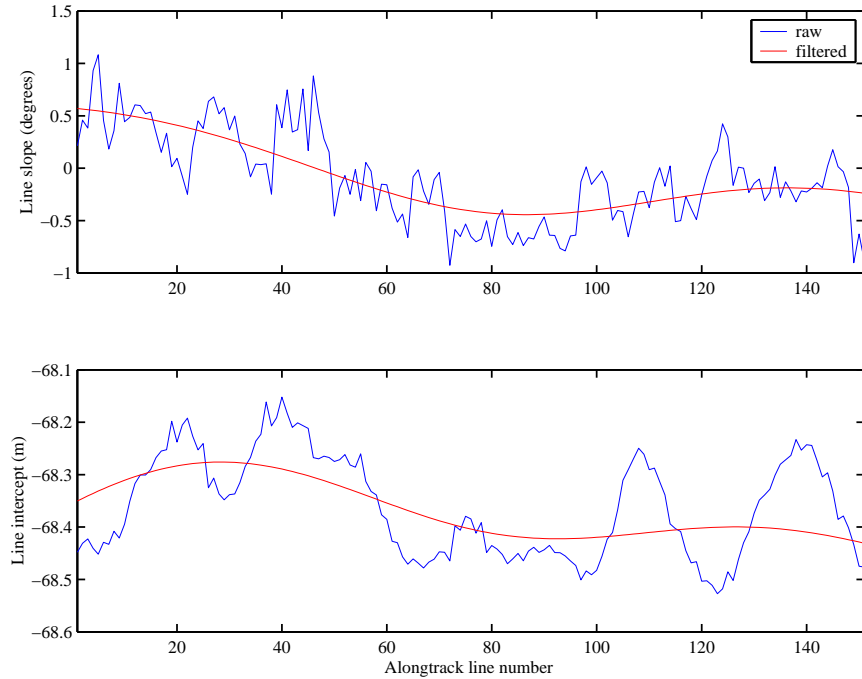
Figure 3: Raw and filtered line slopes and intercepts for the sample of data shown in Figure 2.
