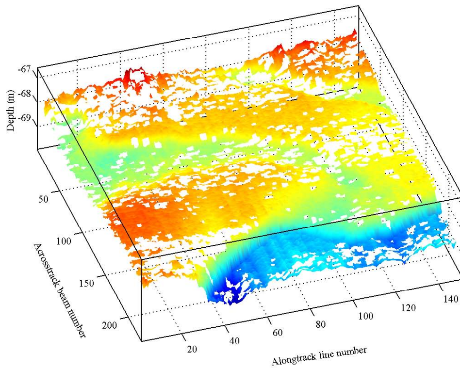
Figure 4: The results of cleaning the data that was shown in Figure 2.
