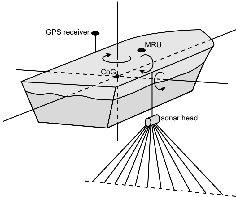
Figure 1: 3-dimensional view of a vessel-mounted multibeam system. Rotation and translation of the vessel are about the CoG. Position is measured at the GPS receiver and attitude, at the MRU.
