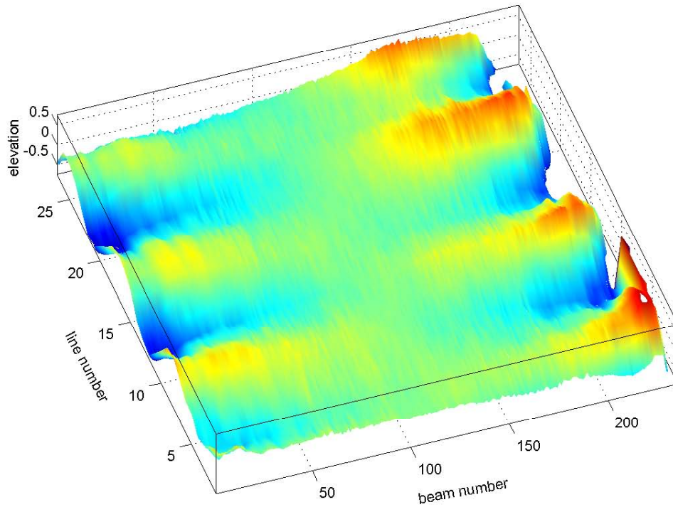
Figure 7: Raw Reson bathymetry data showing motion contamination.
