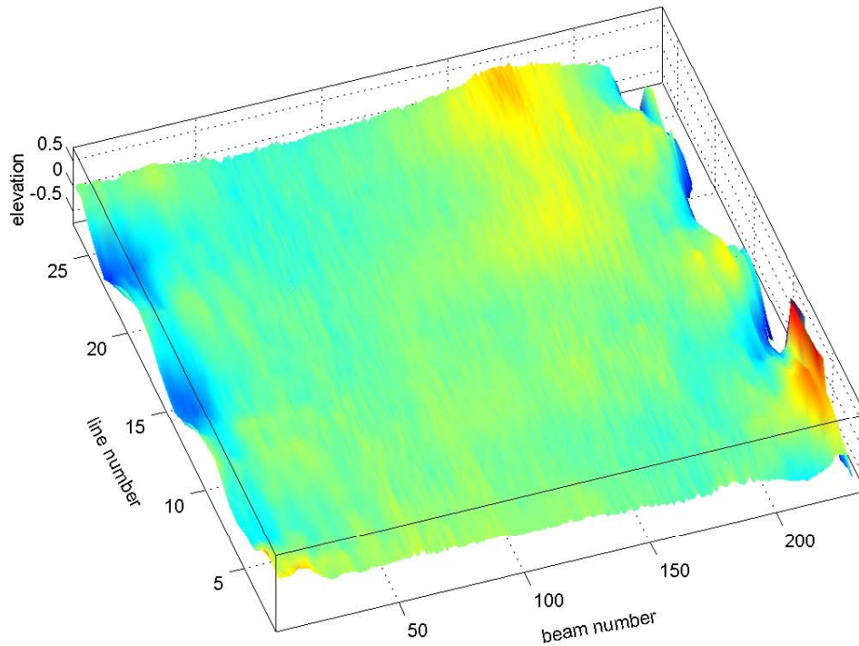
Figure 8: Results of cleaning the data shown in Figure 7. Note the persistence of alongtrack deviation in the outer beams.
