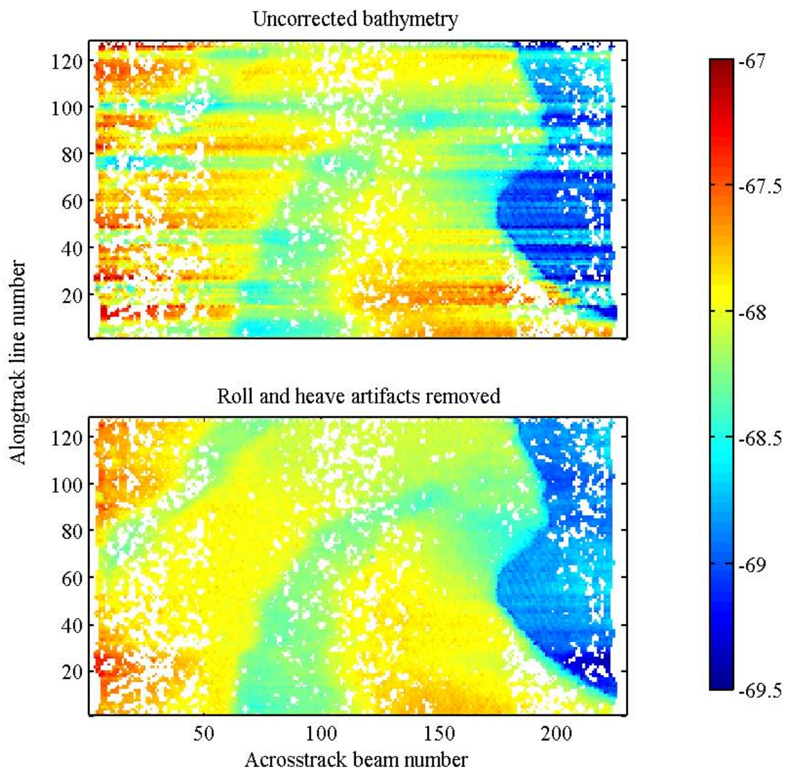
Figure 5: Plan views of the contaminated and cleaned bathymetry data shown in Figures 2 and 4.
