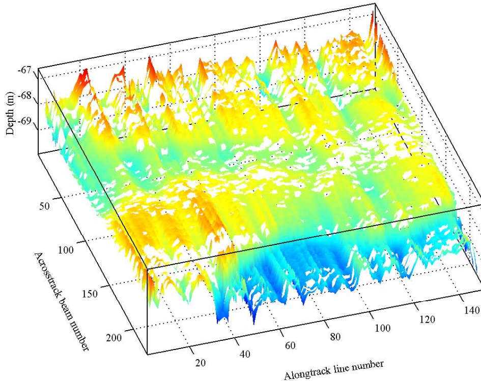
Figure 2: An example of roll and heave contaminated bathymetry data. The mean water depth is 68 meters.
