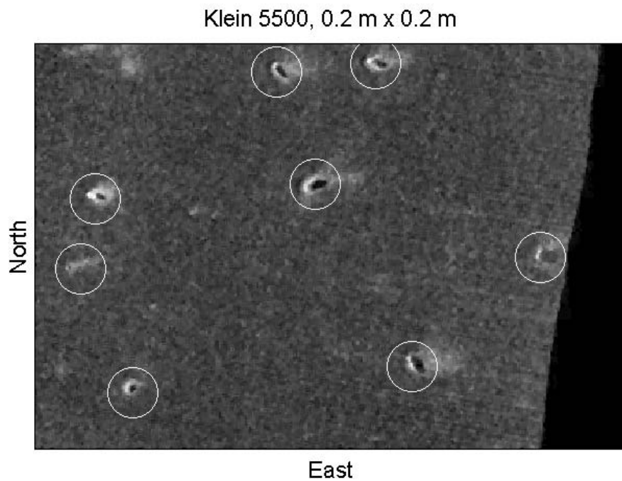
Figure 6: A cluster of mine-shaped targets in cleaned, geo-referenced bathymetry data and in sidescan sonar data over the same area.
