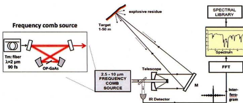
Standoff trace detector based on mid-infrared frequency comb. The mid-infrared 'signature' spectrum is obtained from the time-domain interferogram from a photodetector.
