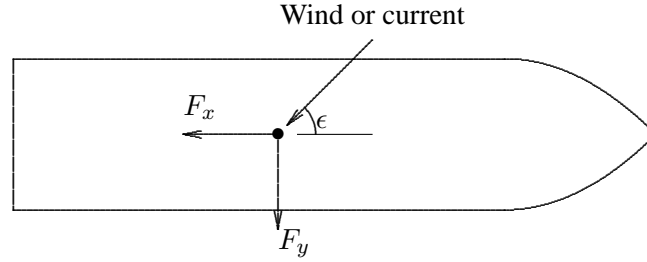
Figure 1: Axis System for Wind and Current Forces
