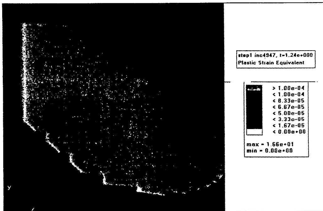
Figure 10 Continued: von Mises Stress and Equivalent Plastic Strain Development, in DT-350WT Specimen with Rising Stress-Strain Curve Model (e) von Mises Stress and (f) Plastic Strain at 16.00 kN (1.08 P_L )
