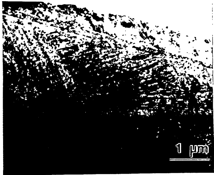
Figure 7. Transmission electron micrograph of remelted material on Alloy 21 revealing a predominately two-phase microstructure of martensite (dark irregular plates) and \alpha (light rod like features). A high density of cuboidal Fe/Cr-rich precipitates is also present.
