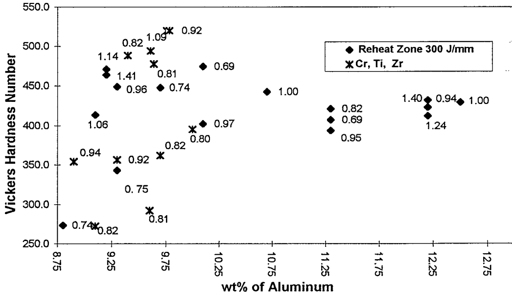
Figure 2. Remelted (a) and reheated (b) zone hardness as a function of aluminum content
