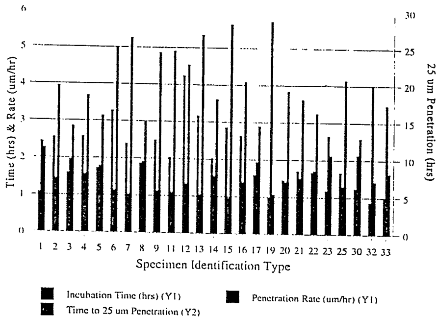
Figure 9. Cavitation erosion behavior
