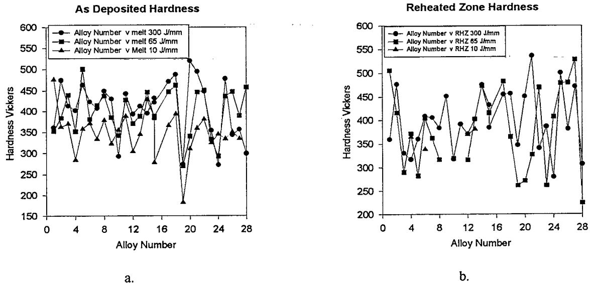
Figure 1. Hardness of as deposited (a) and reheated zones (b) as a function of heat input.
