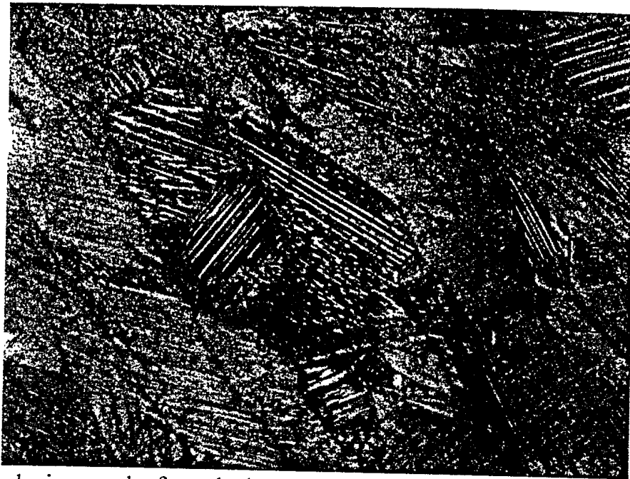
Figure 4. Optical micrograph of remelted material on Alloy 16 which contained 11.3-Al, 4.1-Ni, 5.0-Fe, 1.0 Mn.
