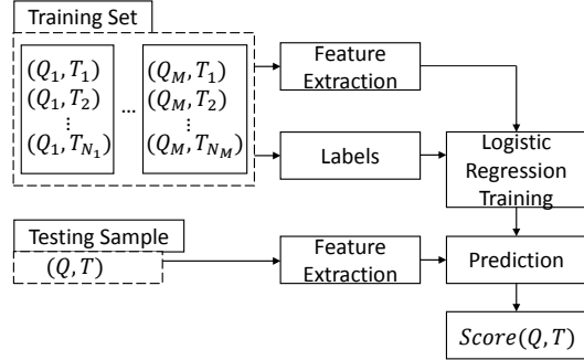
Figure 2: Relevance Prediction Framework
