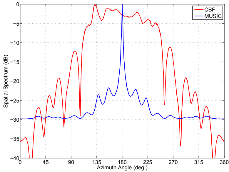
Figure 46: Measured wide-spacing microstrip patch array spatial spectrum for a 1.7 GHz incoming signal at 180^\circ for the classic beamformer and MUSIC algorithms.
