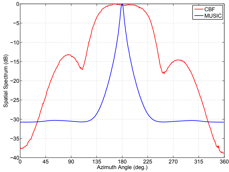
Figure 45: Measured narrow-spacing microstrip patch array spatial spectrum for a 1.7 GHz incoming signal at 180^\circ for the classic beamformer and MUSIC algorithms.
