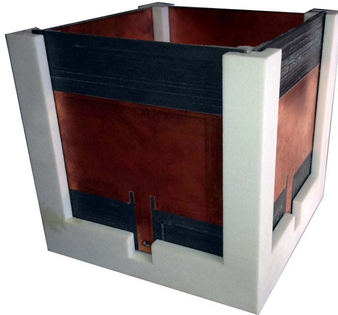
Figure 27: Photograph of the narrow-spacing microstrip patch array in 3D printed mount.
