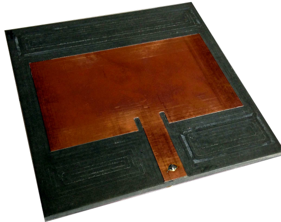
Figure 23: Photograph of a microstrip patch antenna element.
