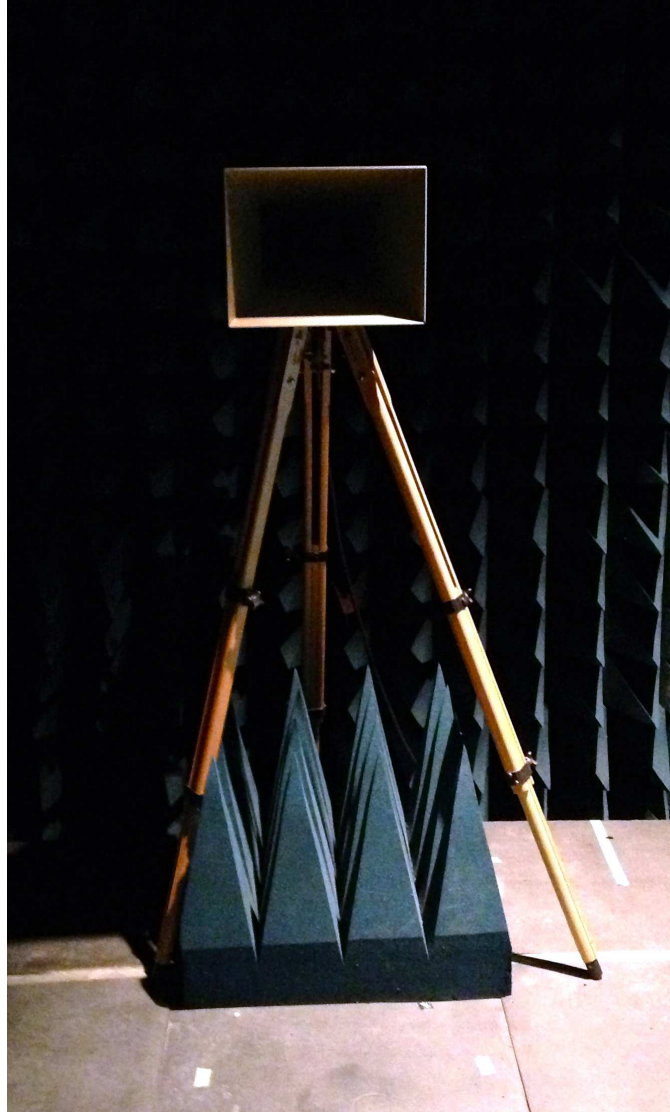
Figure 34: Standard gain horn antenna (ETS-Lindgren model 3160-03) used as the transmitter in the anechoic chamber. The flat surface upon which the antennas are mounted are walkway absorbers (i.e., RAM with a flat support structure on top).
