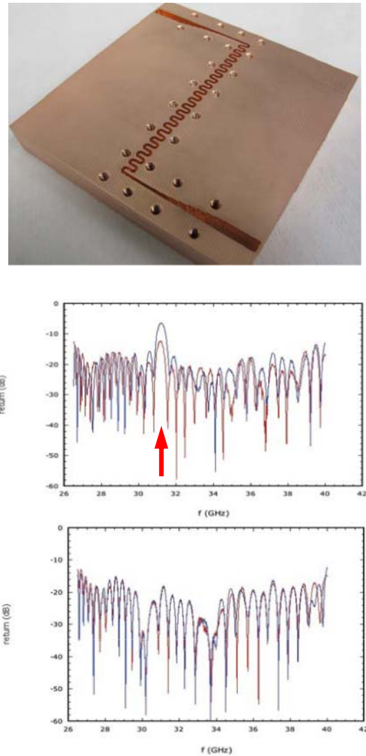
Fig. 8. S_{11} (dB) versus frequency cold-test circuits: early tests without beam tunnel (top, with 3\pi/2 mode marked with arrow) and later results with beam tunnel (bottom).
