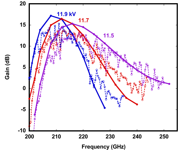
Fig. 10. Small-signal frequency response comparisons between MAGIC predictions (solid) and test data (dashed with symbols) for three beam voltages.
