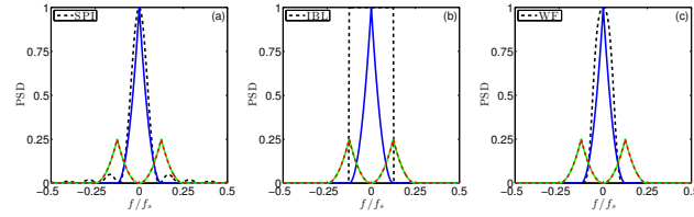
Figure 4.9: An illustration of the frequency response of (a) the sliding pseudo inverse, (b) the ideal band-limited filter, and (c) a Wiener filter (smooth band-limited filter) compared to the graphical representation of the spectral density response of the S_0 channel.
