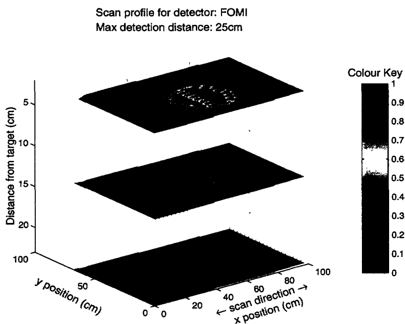
Figure 78: Scan profiles for the FOERSTER Minex 2FD 4.400.01 detector (FOMI). Locked scale.
