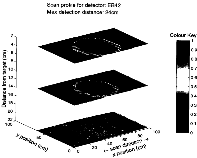
Figure 69: Scan profiles for the Ebinger EBEX 420GC detector (EB42). Unlocked scale.
