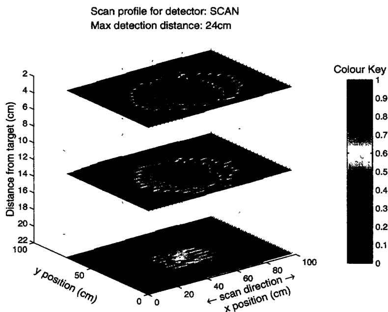
Figure 106: Scan profiles for the Schiebel AN19/2 detector (SCAN). Locked scale.
