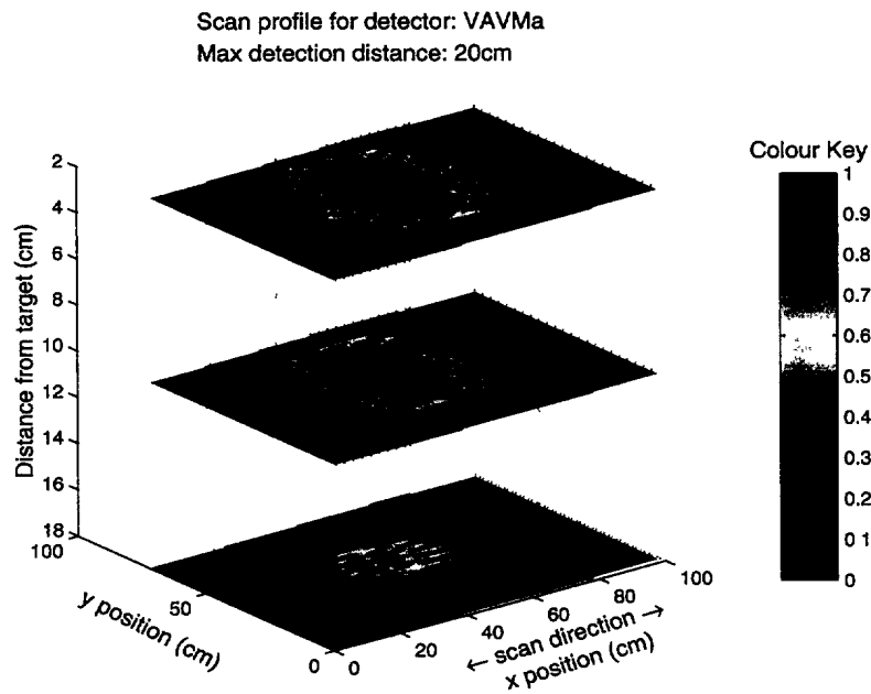
Figure 114: Scan profiles for the Vallon VMH2 detector (VAVMa). Locked scale.
