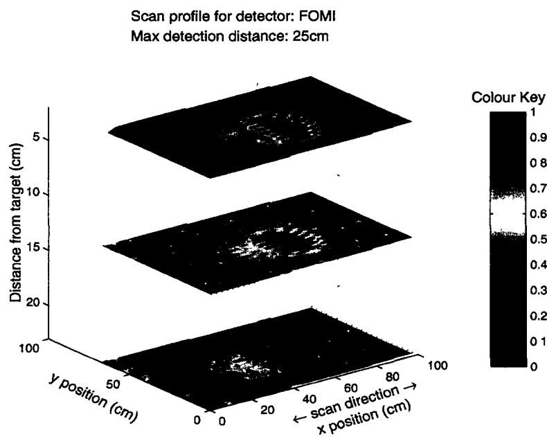
Figure 79: Scan profiles for the FOERSTER Minex 2FD 4.400.01 detector (FOMI). Unlocked scale.
