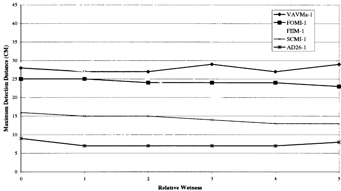
Figure 19: Maximum detection distance vs wetness of detector head for selected detectors (chart 2 of 6).
