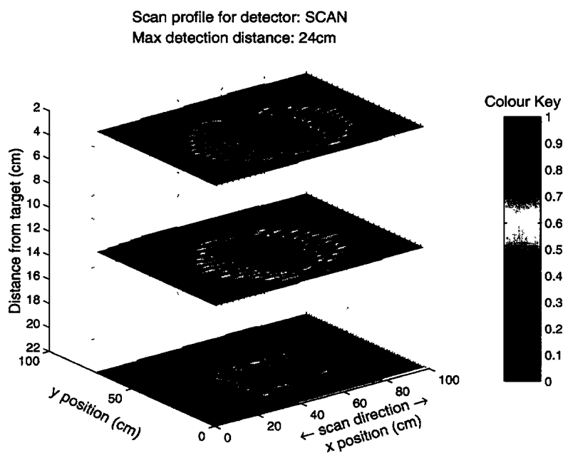
Figure 107: Scan profiles for the Schiebel AN19/2 detector (SCAN). Unlocked scale.
