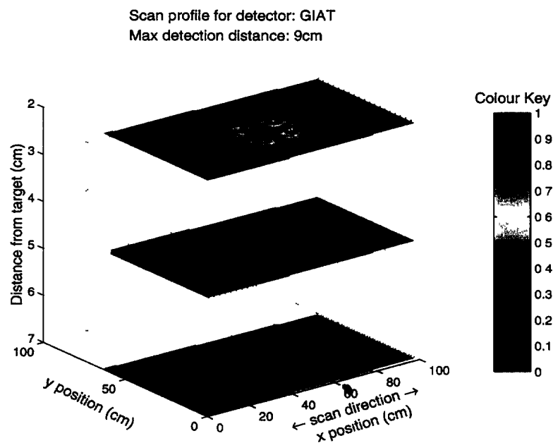
Figure 80: Scan profiles for the GIAT F1 detector (GIAT). Locked scale.
