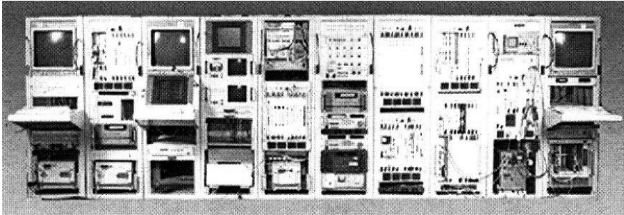
Figure 21. Brassboard ARPDD signal processing system
