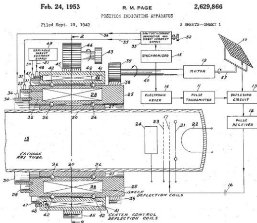
Targets are displayed with their ranges proportional to the radial distance from the center and their bearings by their angular positions. (U.S. Patent 2,629,866). 120,121
