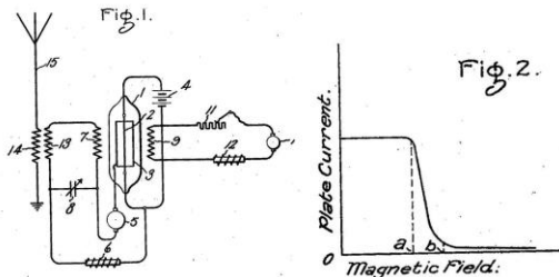
Nov. 23, 1926. A. W. HULL 1,608,316 METHOD OF AND MEANS FOR PRODUCING ALTERNATING CURRENTS Filed Jan. 29, 1920
