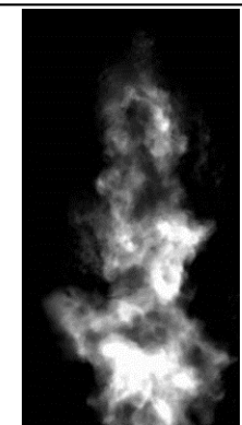
H 2 /O 2 Reacting Coaxial Jet
