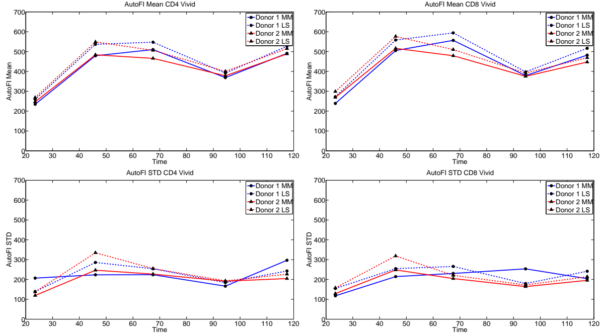
Figure 5: Top: Mean autofluorescence as estimated by the method of moments (solid lines) and least squares (dashed lines). Bottom: Standard deviation as estimated by the method of moments (solid lines) and least squares (dashed lines). Data shown for CD4 T cells (left) and CD8 T cells (right). Mean autofluorescence is observed to increase significantly in the first two days of the experiment, an effect which is known to be the result of cellular activation. The cause of the decrease in mean autofluorescence at approximately 96 hours is unknown; nutrient depletion is one hypothesized cause.
