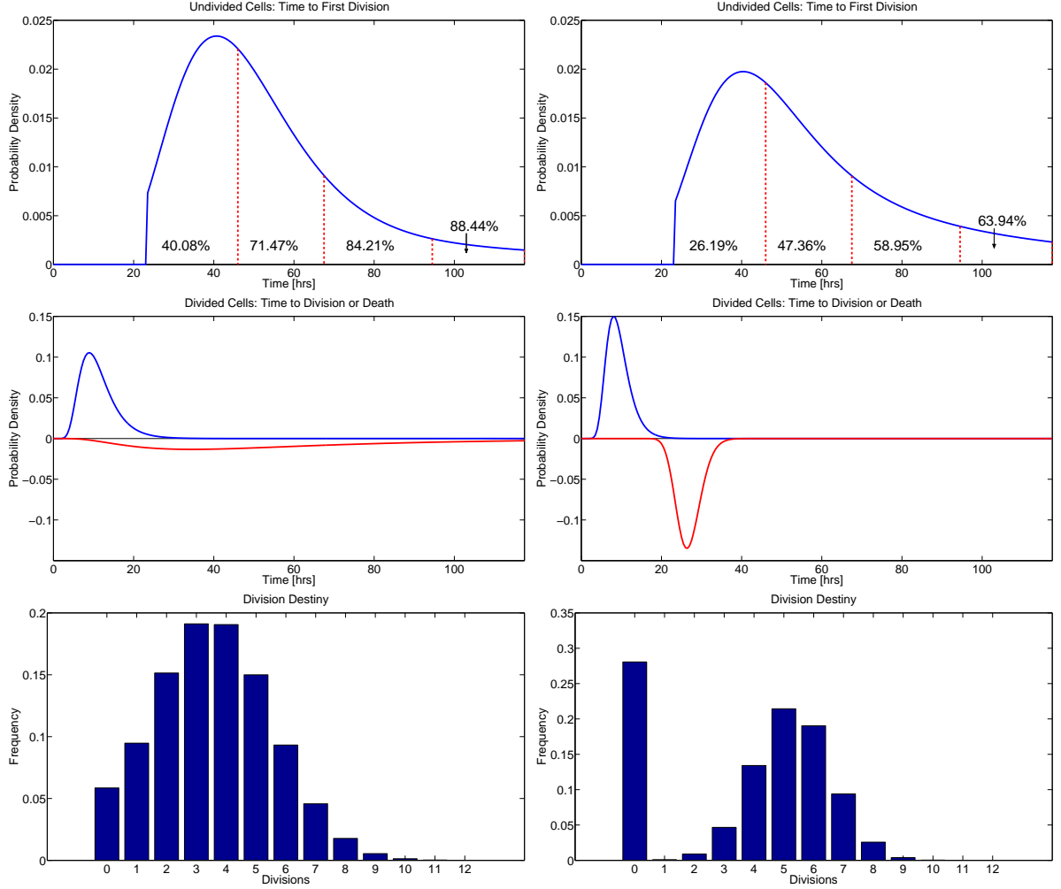
Figure 9: Comparison of estimated CD8 T cell division dynamics between Donor 1 (left) and Donor 2 (right). Top: Probability density function \phi_0(t) for time to first division for initially undivided CD8 T cells, scaled by the initial progressor fraction F_0 of activated cells. Percentages indicate the fraction of undivided cells which will have entered their first division by the next measurement time (vertical dashed lines). On average, cells for Donor 1 complete their first division more rapidly than those for Donor 2 and cells from Donor 1 are more likely to have divided in response to stimulus before the end of the experiment. Middle: Probability density functions for time to subsequent division or time to die (inverted) for CD8 T cells having completed at least one division. Cells from Donor 2 divide slightly more rapidly and more synchronously than those from Donor 1. Bottom: Division destiny, indicating the average number of divisions undergone by cells initially in the population (at t = t_0 ). The fraction of cells with division destiny equal to zero estimates the relative abundance of cells which will not become activated to divide.
