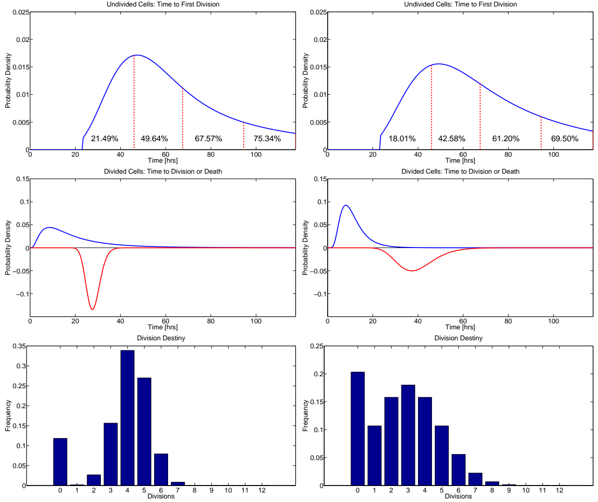
Figure 8: Comparison of estimated CD4 T cell division dynamics between Donor 1 (left) and Donor 2 (right). Top: Probability density function \phi_0(t) for time to first division for initially undivided CD4 T cells, scaled by the initial progressor fraction F_0 of activated cells. Percentages indicate the fraction of undivided cells which will have entered their first division by the next measurement time (vertical dashed lines). On average, cells for Donor 1 complete their first division more rapidly than those for Donor 2; cells from Donor 1 are also more likely to have divided in response to stimulus before the end of the experiment. CD4 T cells from both donors are estimated to respond more slowly and in greater frequency than CD8 T cells (compare Figure 9). However the total CD 8 T cell response for Donor 1 is greater than the CD4 T cell response while the total CD4 and CD8 responses are comparable for Donor 2. Middle: Probability density functions for time to subsequent division or time to die (inverted) for CD4 T cells having completed at least one division. Cells from Donor 2 divide slightly more rapidly and more synchronously than those from Donor 1. Bottom: Division destiny, indicating the average number of divisions undergone by cells initially in the population (at t = t_0 ). The fraction of cells with division destiny equal to zero estimates the relative abundance of cells which will not become activated to divide.
