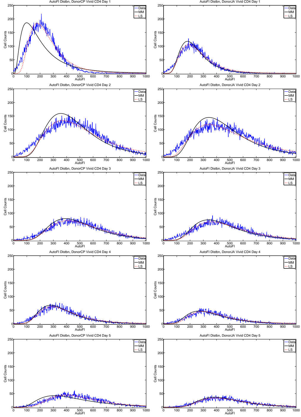
Figure 3: Measured autofluorescence distributions in comparison to fitted lognormal curves for Donor 1 (left) and Donor 2 (right) for CD4 T cells. The least squares fit (LS) to data is visually better than the fit obtained by the method of moments (MM), though the difference is small and becomes less noticeable at later measurement times. This pattern is more noticeable for CD4 T cells (here) than for CD8 T cells (Figure 4).
