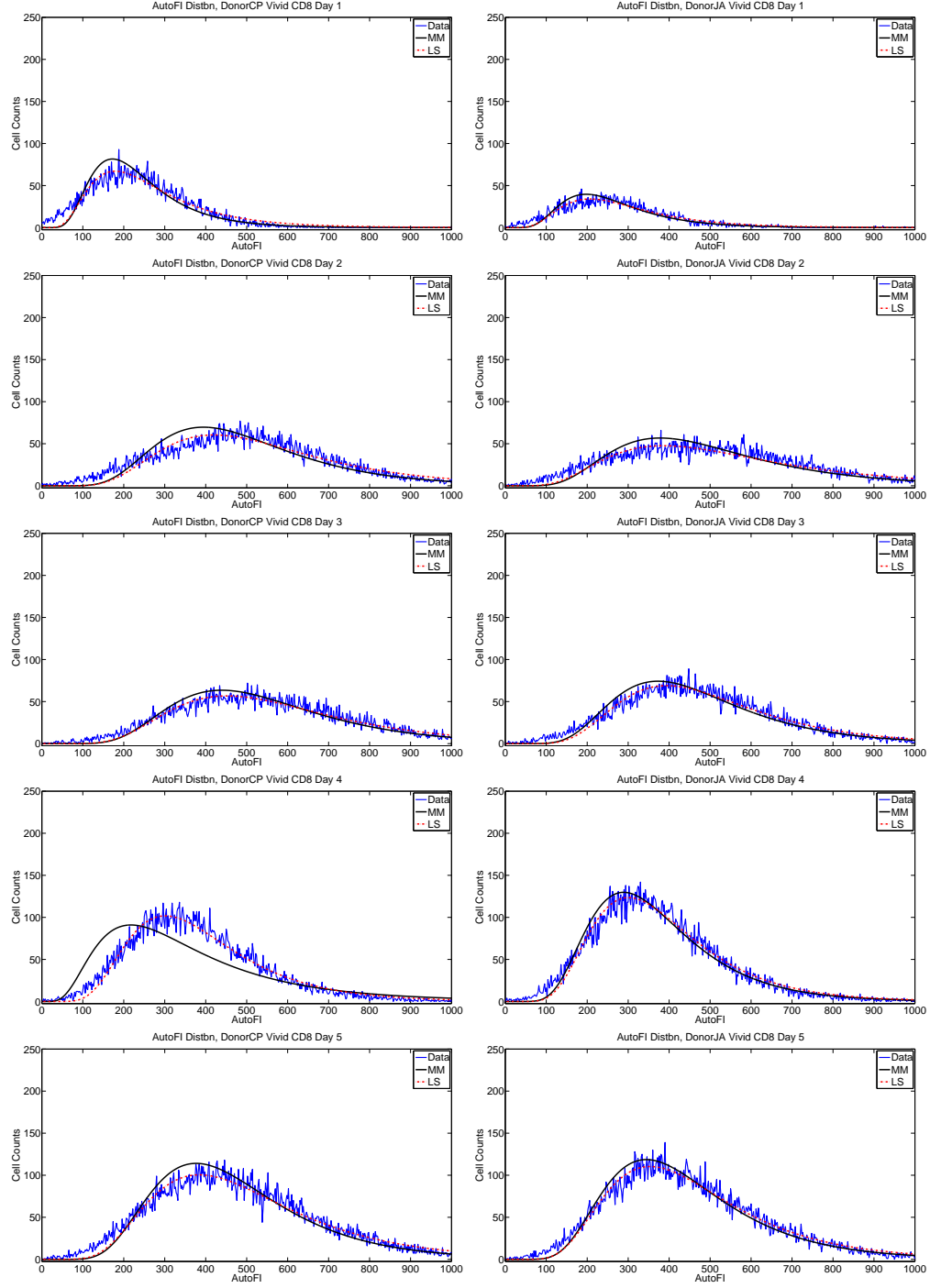
Figure 4: Measured autofluorescence distributions in comparison to fitted lognormal curves for Donor 1 (left) and Donor 2 (right) for CD8 T cells. The least squares fit (LS) to data is visually better than the fit obtained by the method of moments (MM), though the difference is small.
