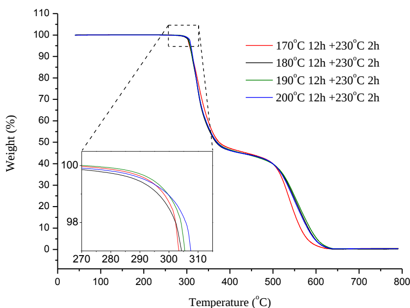
Figure 2.14 Thermogravimetric analysis of resins cured at different temperatures.
