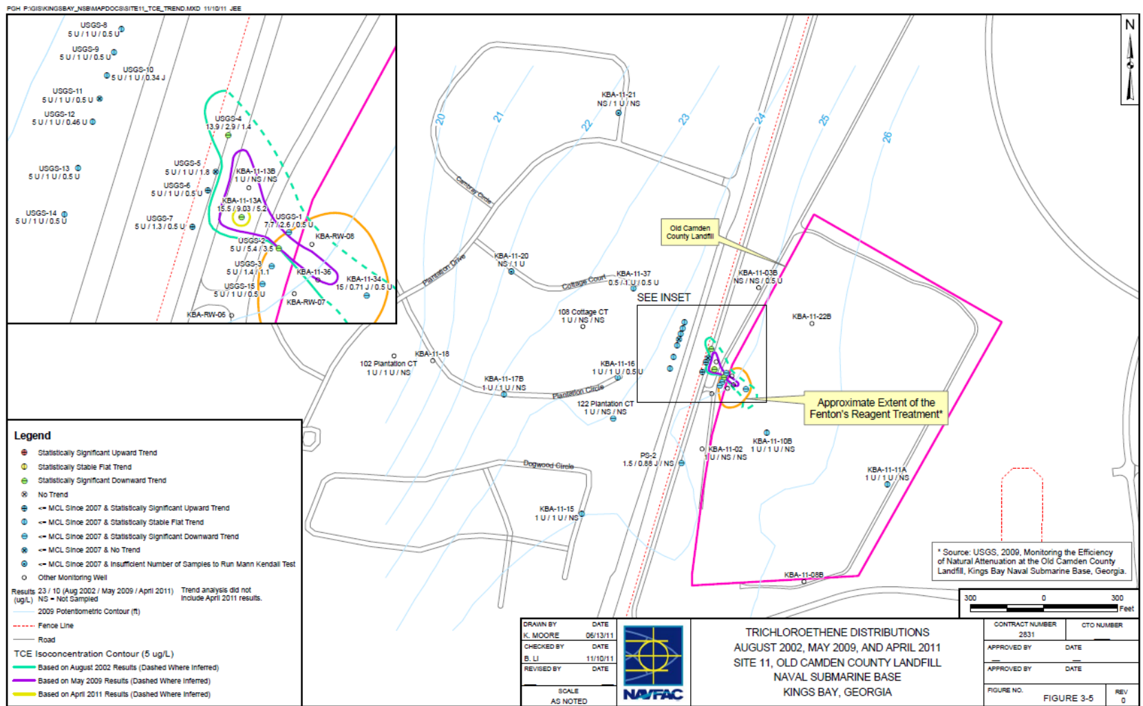
Figure 4.11: Trichloroethene distribution in August 2002, May 2009, and April 2011, Site 11, Old Camden Landfill, Kings Bay, Georgia.
