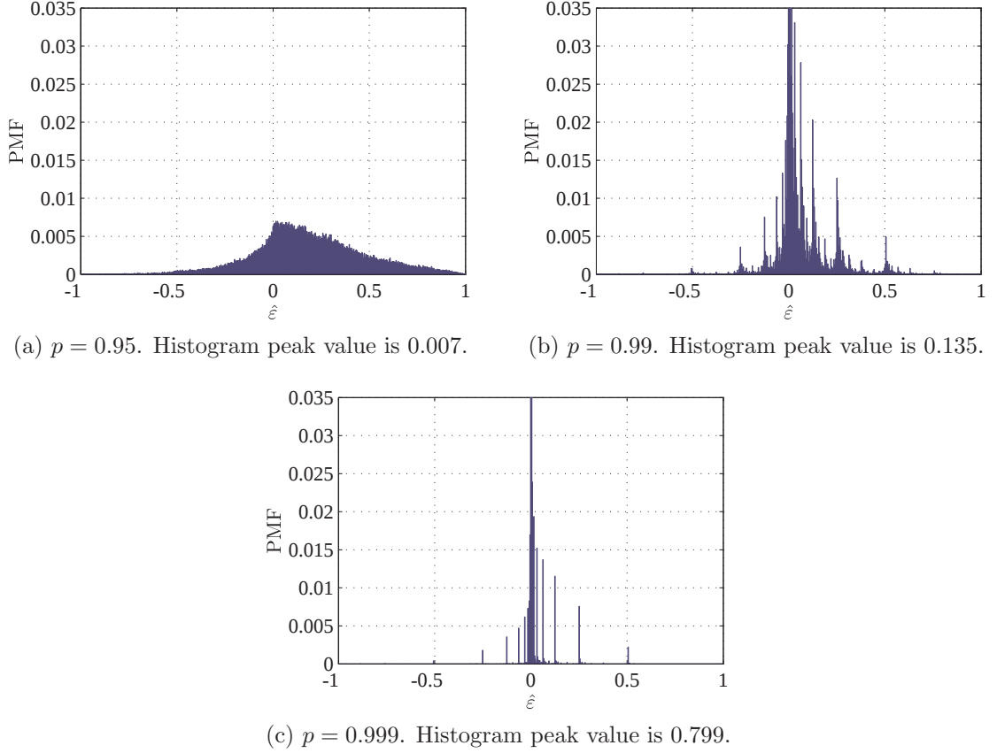
Figure 35. Error histograms for an inexact 16-bit Wallace tree multiplier, with inputs A and B uniformly distributed from 0 to 2^N - 1 , for various values of p . Results are from Matlab PBL simulation.
