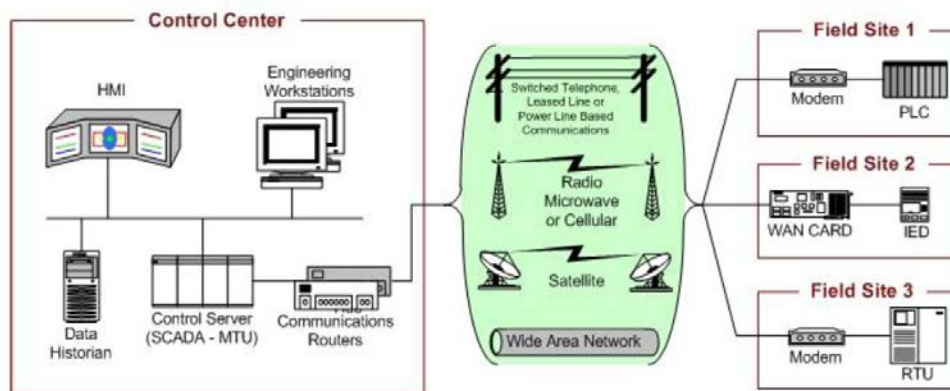
Figure 3. SCADA System General Layout 2014.
