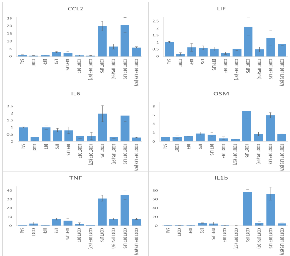
Figure 5: 90 and 97d GWI model - Results on cytokine expression in the cortex at 90 and 97 days.
