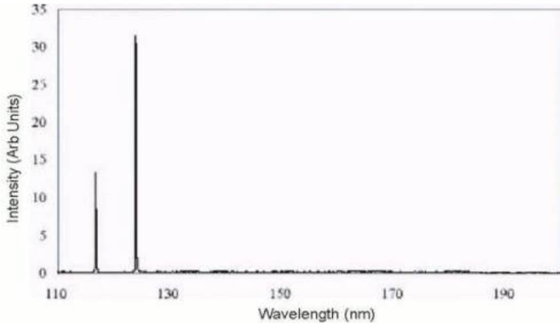
Figure 4: Spectrum of Kr VUV Lamps.
