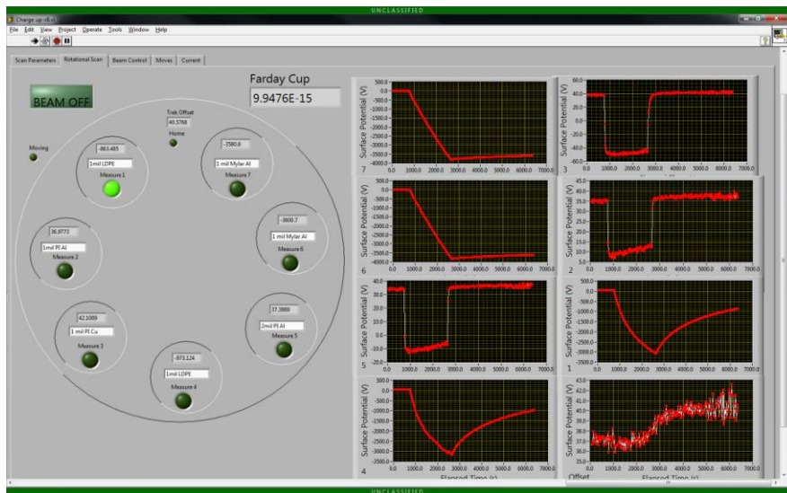
Figure 10: Front Panel of LabVIEW Automated Control Program.
