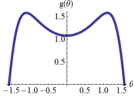
Figure 4: The function g(\theta) plotted above represents the angular dependence of the polarization-rotated field on the incident wave vector's orientation for a specific geometry ( \theta_B = \phi_B = 0 , E_y = 0 ).
