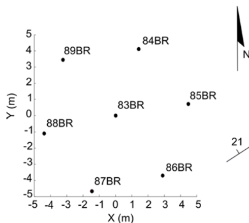
Figure 5.2.1.1: As-built borehole schematic
