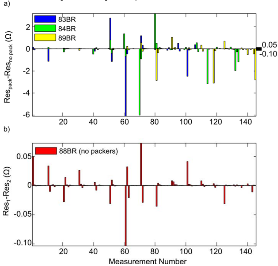
Figure 5.5.1.4: a) Measurements collected with packers inflated ( Res_{\text{pack}} ) and deflated ( Res_{\text{no pack}} ) within single boreholes (83BR, 84BR and 89BR) demonstrate the effect of packers on limiting current flow along the borehole. b) For comparative purposes, the difference between two consecutive datasets ( Res_1 and Res_2 ) where packers were deflated in both cases is shown for 88BR. Note the difference in y-axis scales where the scale of b) is denoted on the right side y-axis a).
