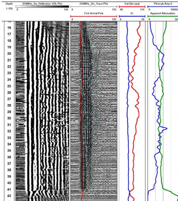
Figure C.4: Single-hole GPR reflection data from BM36 showing the radar data in two left panels and interpretation of first arrival, velocity, dielectric permittivity ( \epsilon_r ), amplitude, and apparent attenuation.
