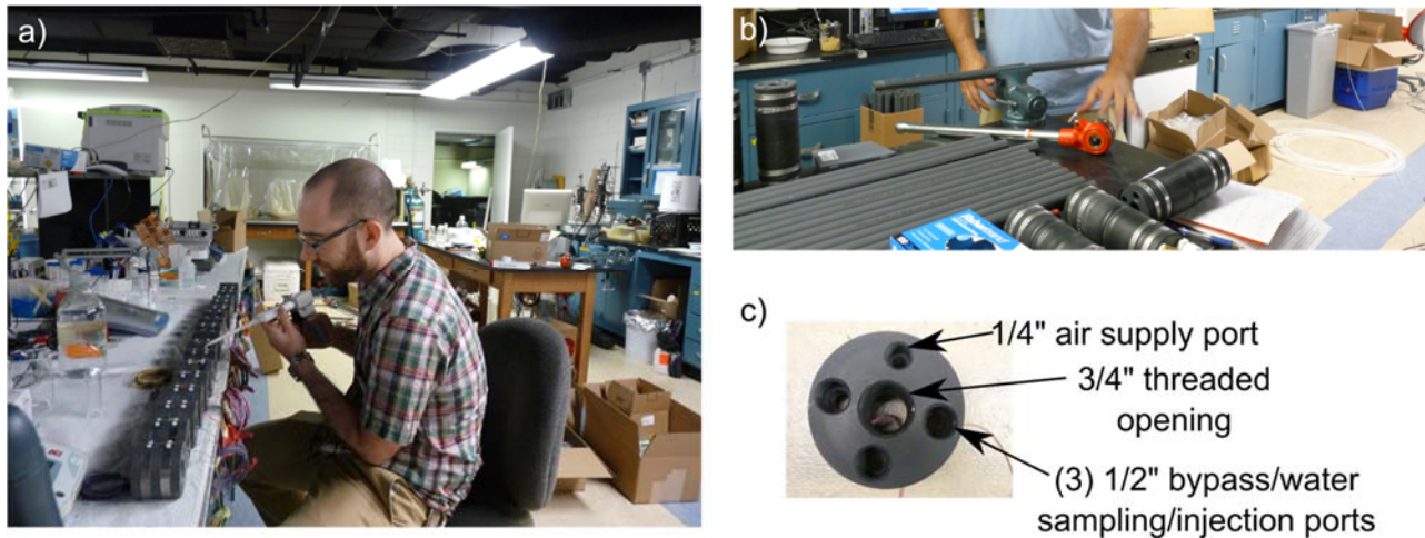
Figure 5.4.8: a) Electrode construction b) Preparation of threaded PVC piping c) Cross section of electrode/packers.
