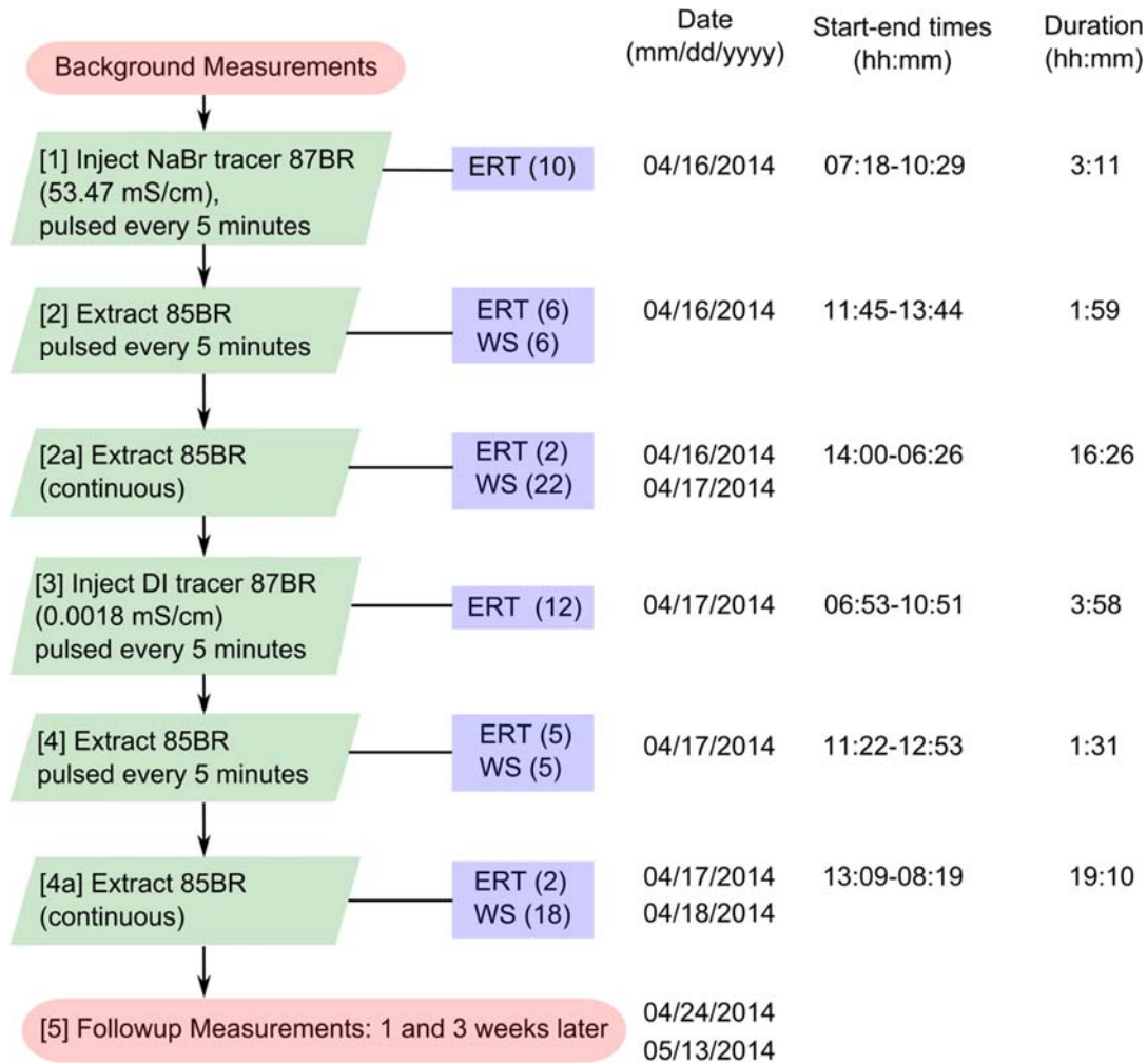
Figure 5.5.3 5: Flow chart of tracer test where numbers of ERT data acquisitions and water samples (WS) are indicated in parentheses ( ).
