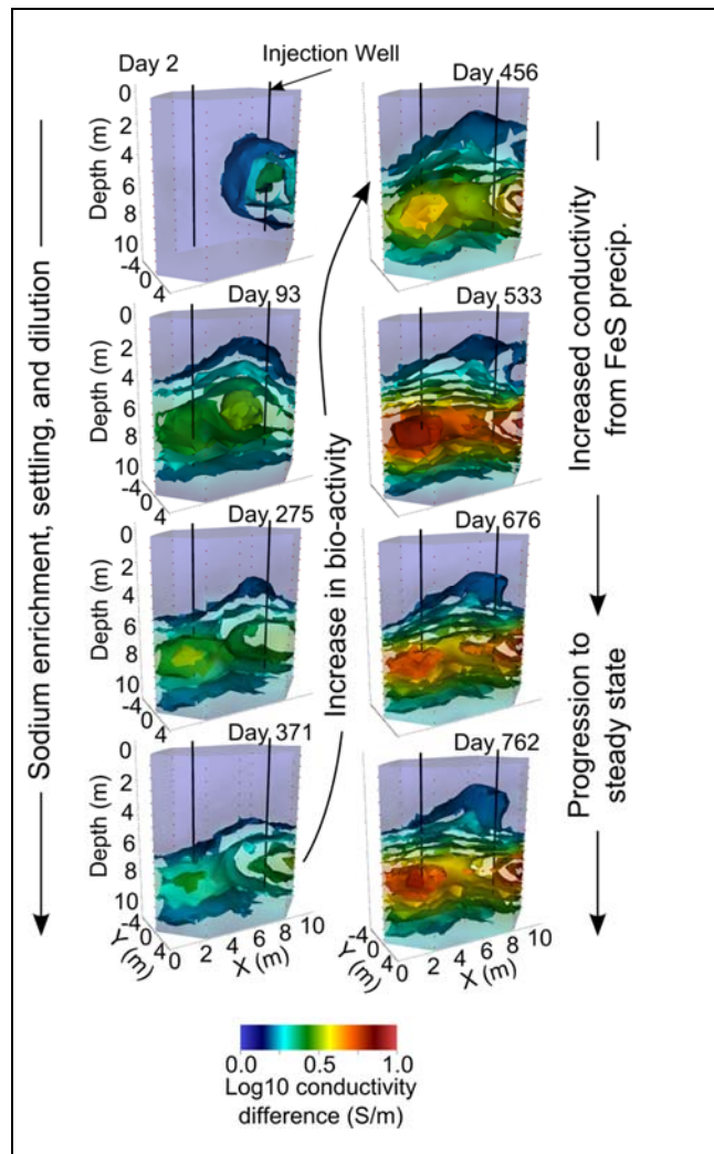
Figure 2. 7. Example 3D time-lapse ERT images from the ESTCP ER-0717 project showing bioamendment (ABC) emplacement and movement, seen as increased bulk electrical conductivity (first column), followed by later increase in bulk conductivity arising from FeS precipitation resulting from microbial activity (second column). The Brandywine time-lapse ERT work demonstrated the capabilities of electrical imaging to provide near real-time, actionable information to remediation operators in the field. (from Johnson et al., 2014).
