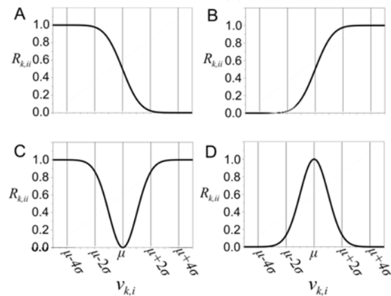
Figure 5.4.5: Reweighting functions in E4D ( https://e4d.pnnl.gov/ ) A) The weighting of v_{k,i} begins to minimize if the value of v_{k,i} drops below \mu+2\sigma , reaching the full weight if v_{k,i} drops below \mu-2\sigma . B) The weighting of v_{k,i} begins to minimize if the value of v_{k,i} rises above \mu-2\sigma , reaching the full
