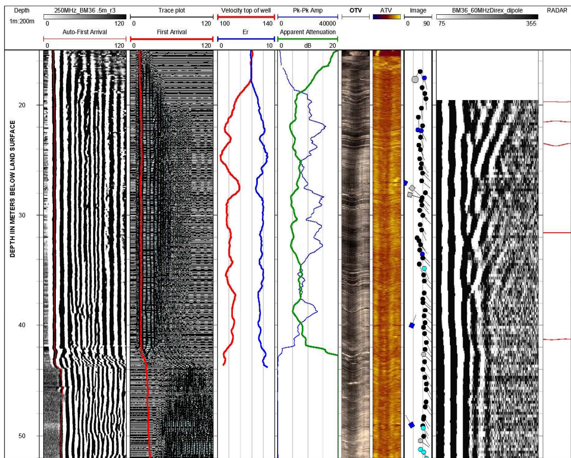
Figure C.7: Single hole GPR data collected in BM36. 250 MHz reflection data, first arrival, velocity, dielectric permittivity (Er), amplitude, and apparent attenuation are shown the four left panels of data. Radar logs can be directly compared to OTV, ATV, and tadpole plots from borehole imaging. The panel on the far right shows the dipole component of the 60-MHz DBHGPR data collected in BM36.
